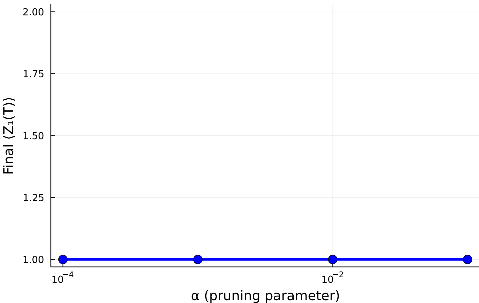
Final Correlation \langle Z_1(T=10) \rangle vs Alpha (N=16)
