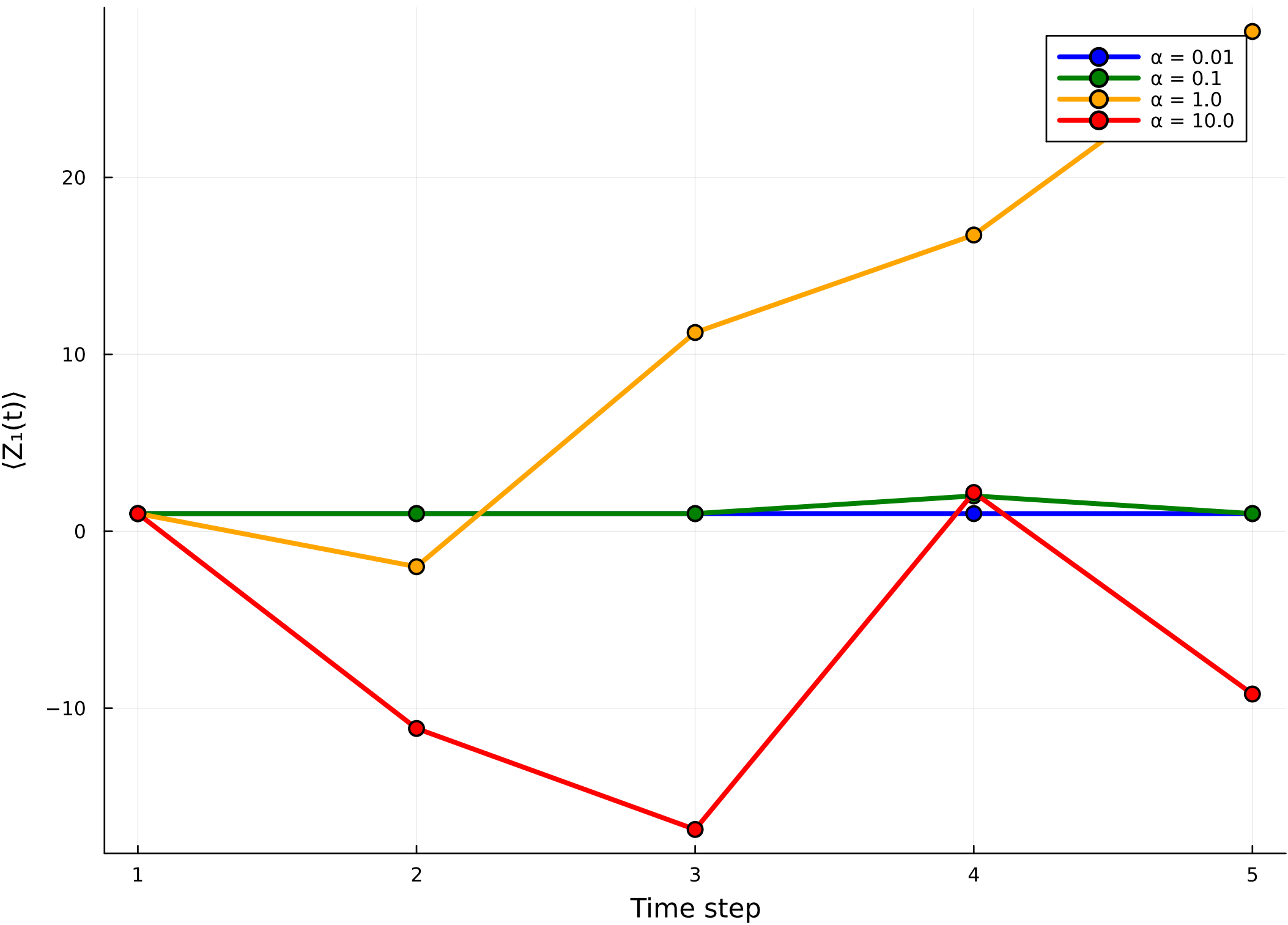
Effect of Alpha Pruning on \langle Z_1(t) \rangle (N=8)
