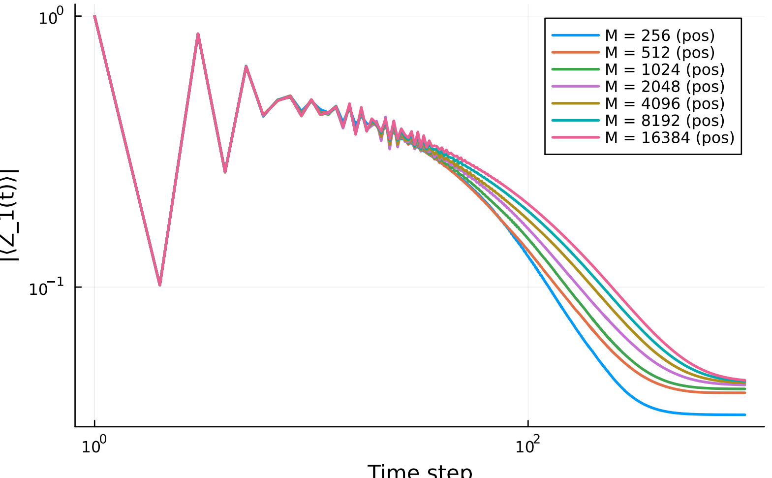
Correlation Function Log-Log (Positive=solid, Negative=dashed)
