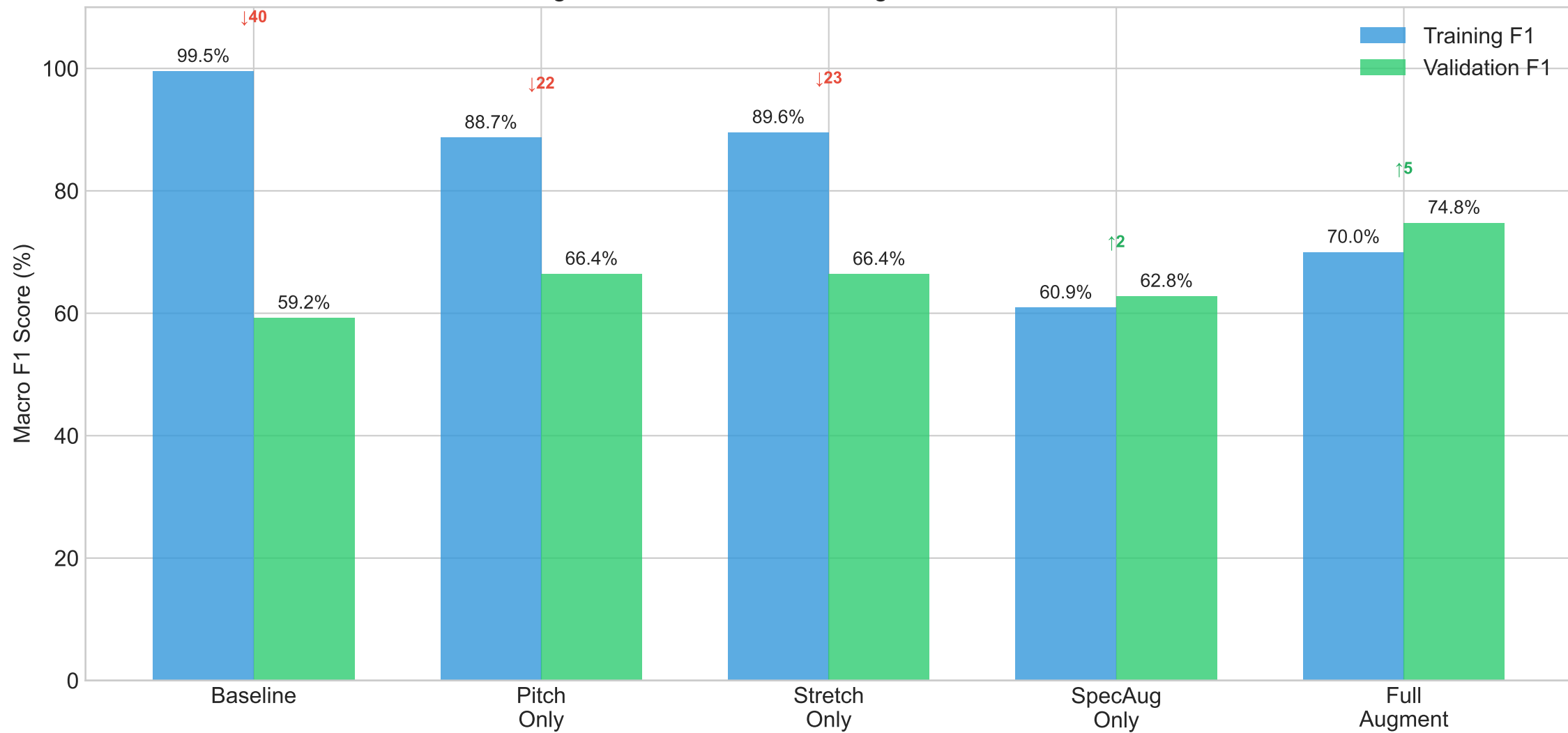
Data Augmentation Ablation: Training vs Validation Performance
