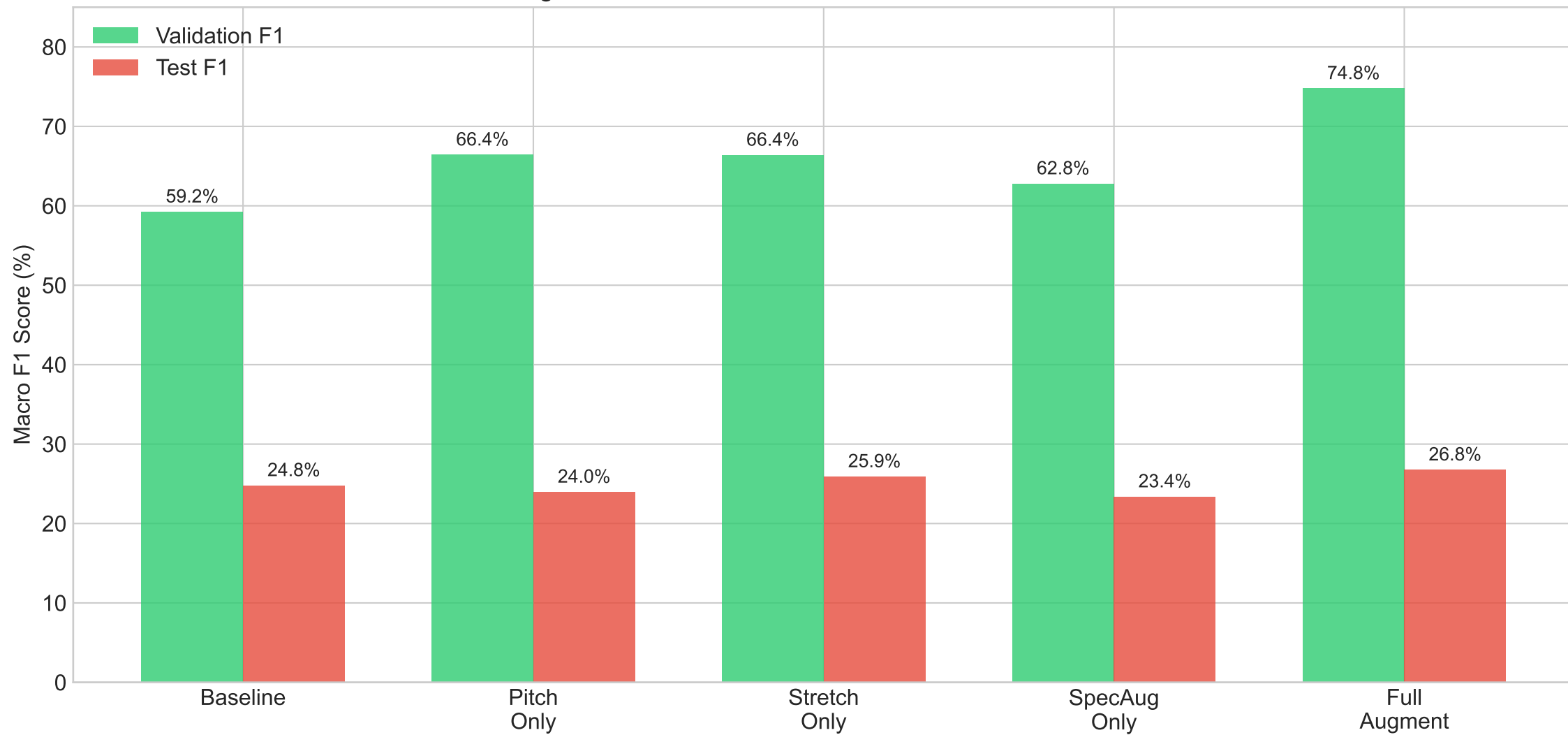
Augmentation Ablation: Validation vs Test Performance
