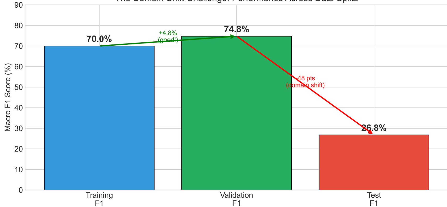
The Domain Shift Challenge: Performance Across Data Splits
