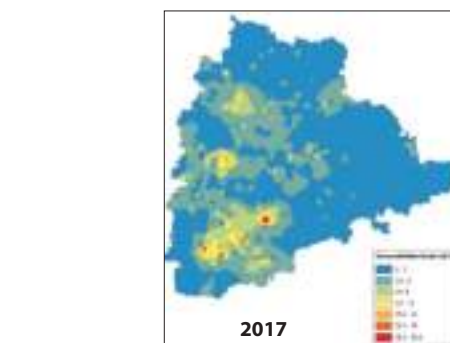
Ground water level variations in Telangana state during 2013-17
