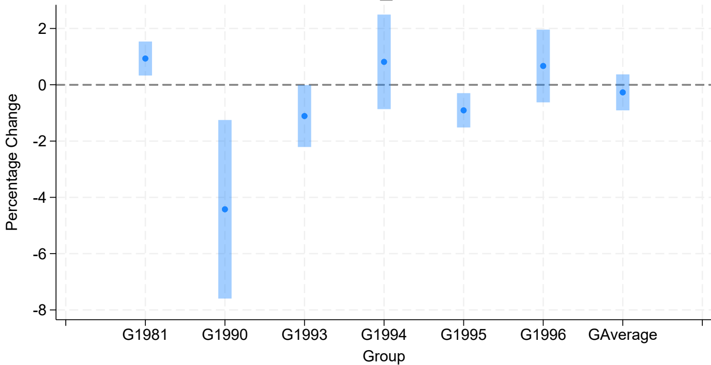
ATT by group: lcit2_wt2
