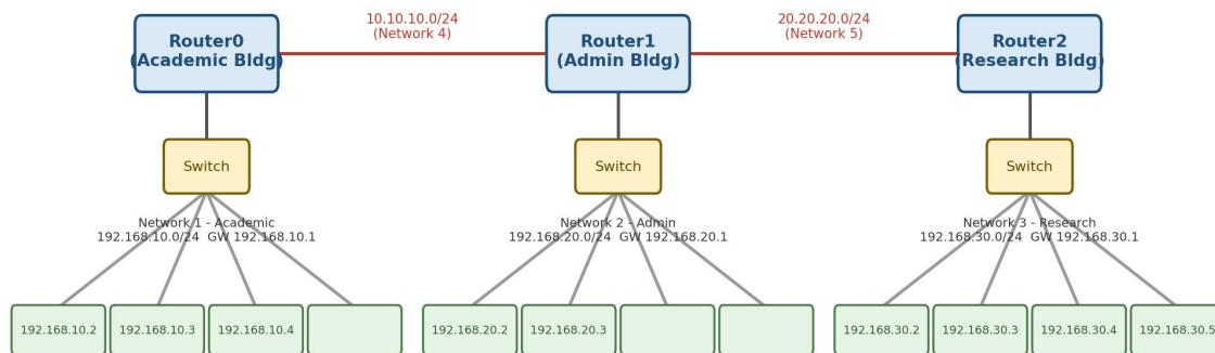
OSPF Design - Linear Backbone (Single Area 0)
