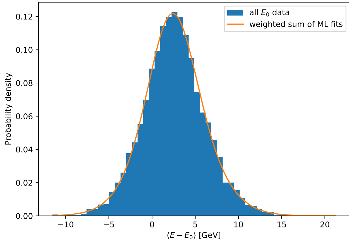
All (E - E_0) overlaid with sum of sub-distributions
