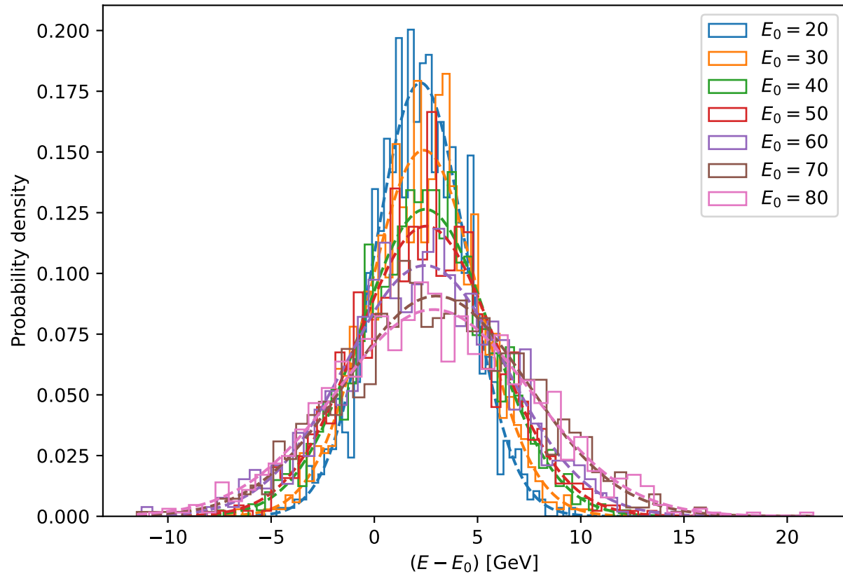
Distributions of (E - E_0) at each E_0 along with ML fits
