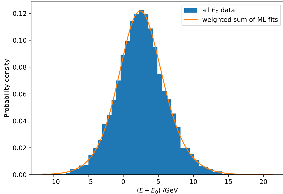
All (E - E_0) overlaid with sum of sub-distributions
