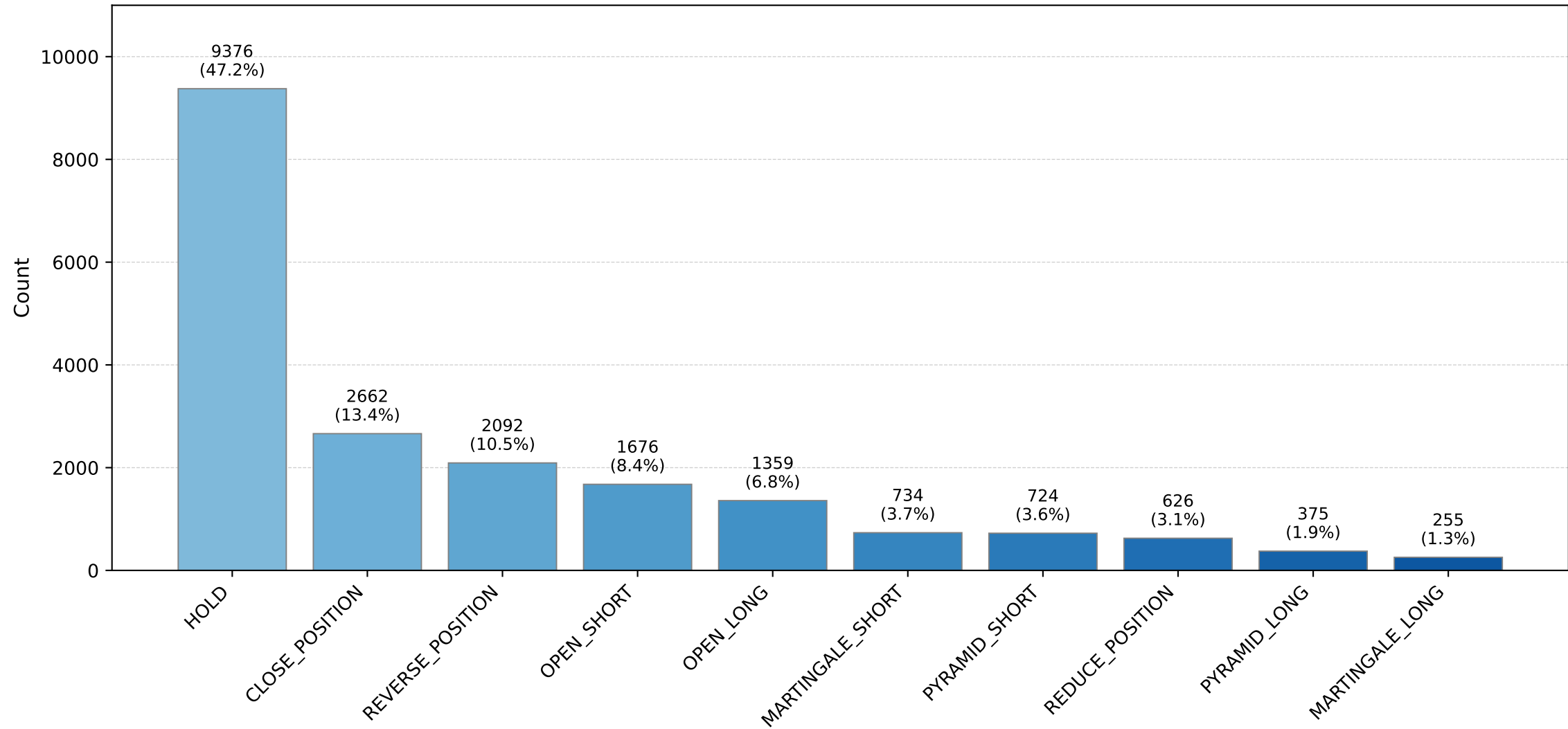
Action Distribution — DoubleDQN EURUSD
