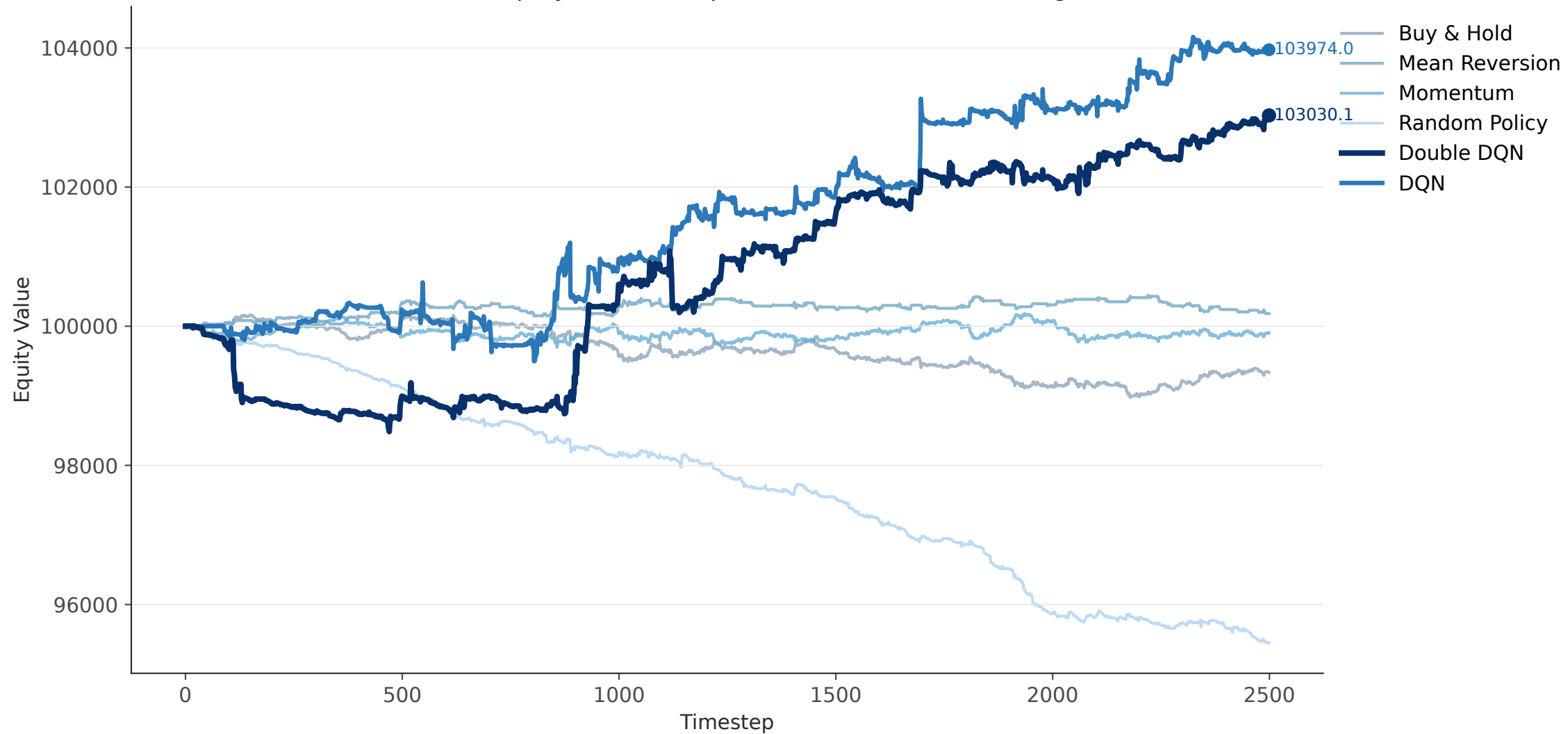
EURUSD — Equity Curve Comparison with Different Strategies
