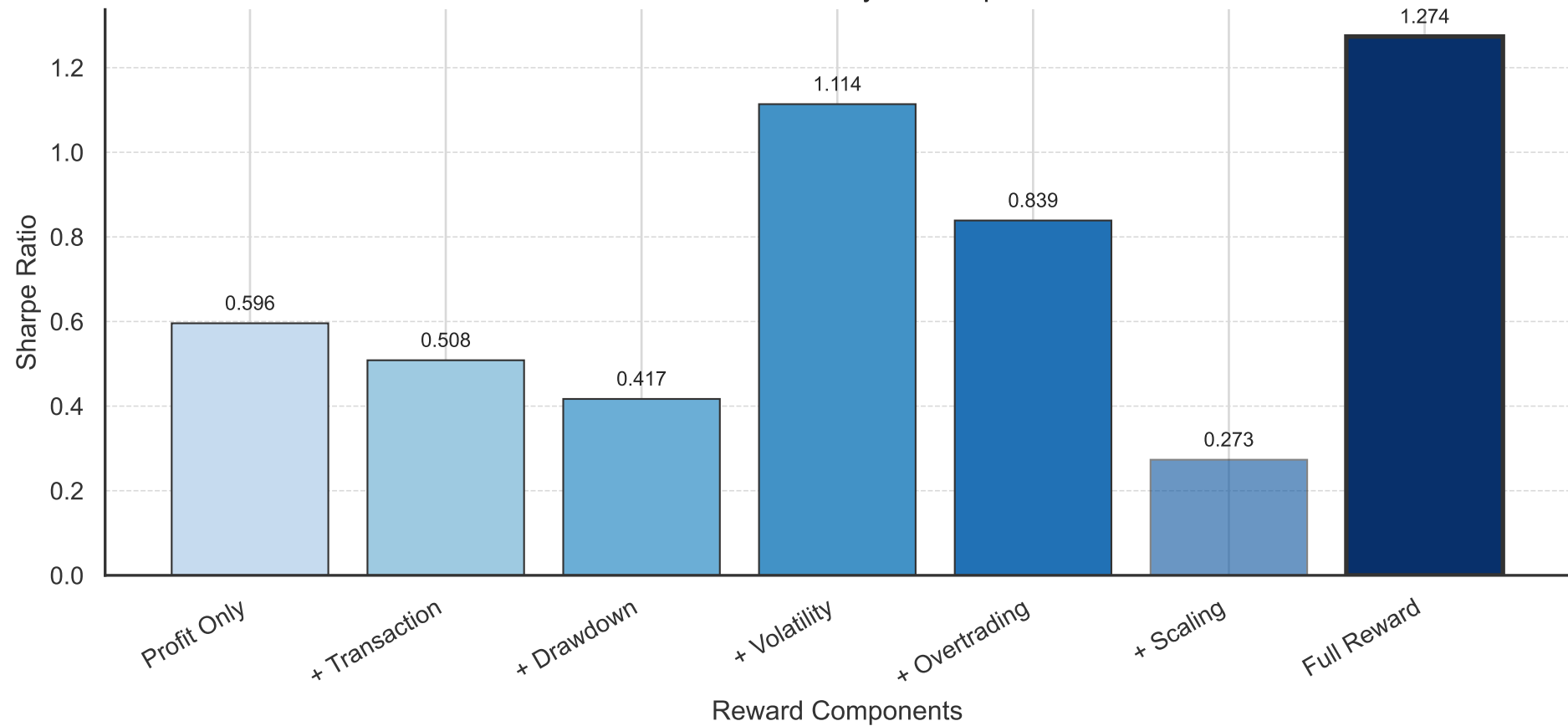
Reward Ablation Study — Sharpe Ratio
