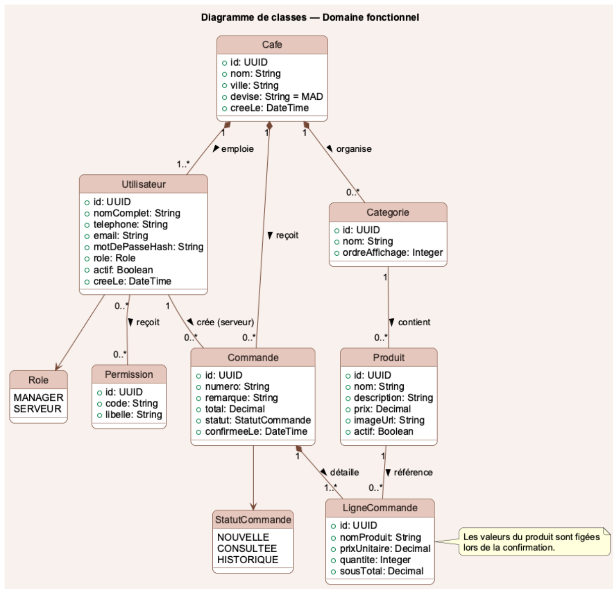
Figure 6 – Diagramme de classes complet.
