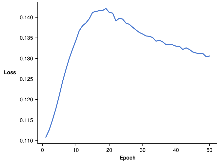
Val Loss
