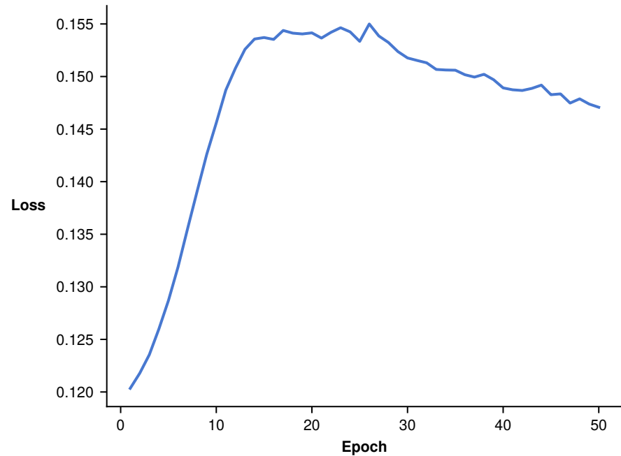
Val Loss
