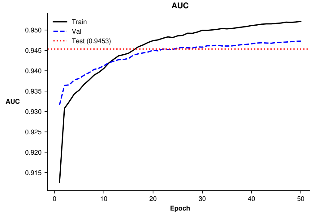
Global learning curves (WHO SNPs)
