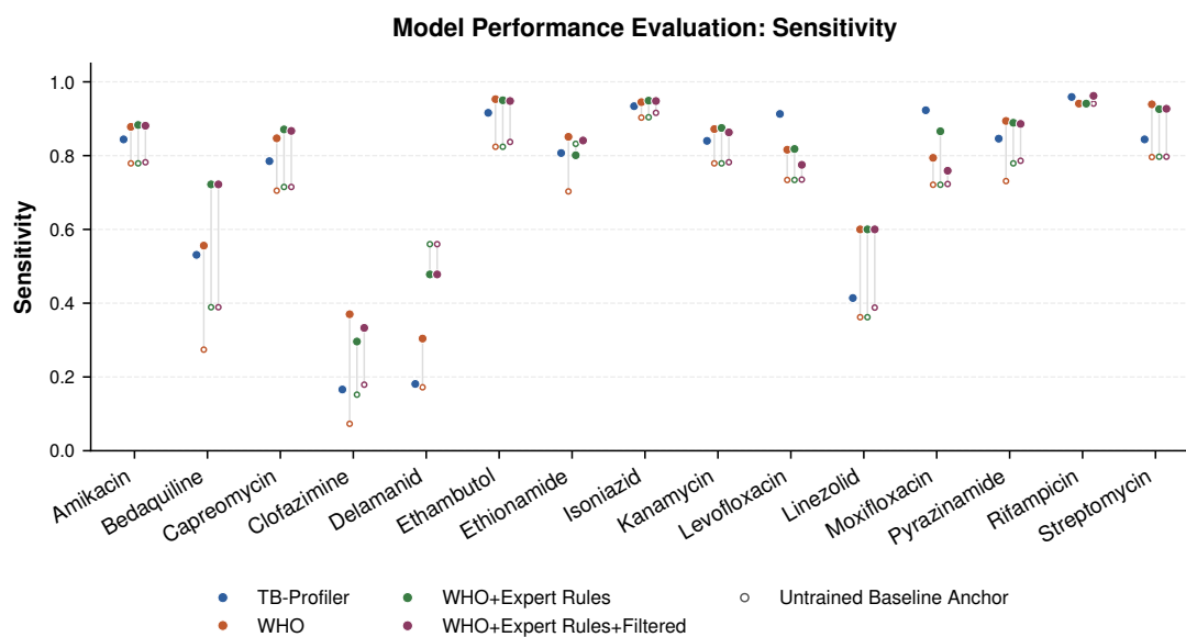
Figure 9: Sensitivity of the neural network with tb-profiler as the baseline, WHO, and WHO augmented with expert rules, and filtered is shown aswell. The naive pass with only the catalogues encoded as 1s , or 0s is shown as empty circles, and the trained model results are filled in.
