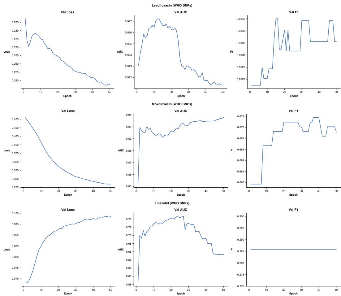
Figure 18: Model performance across all drugs
