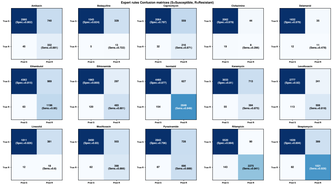
Figure 13: Confusion matrix for er+who catalogue.
