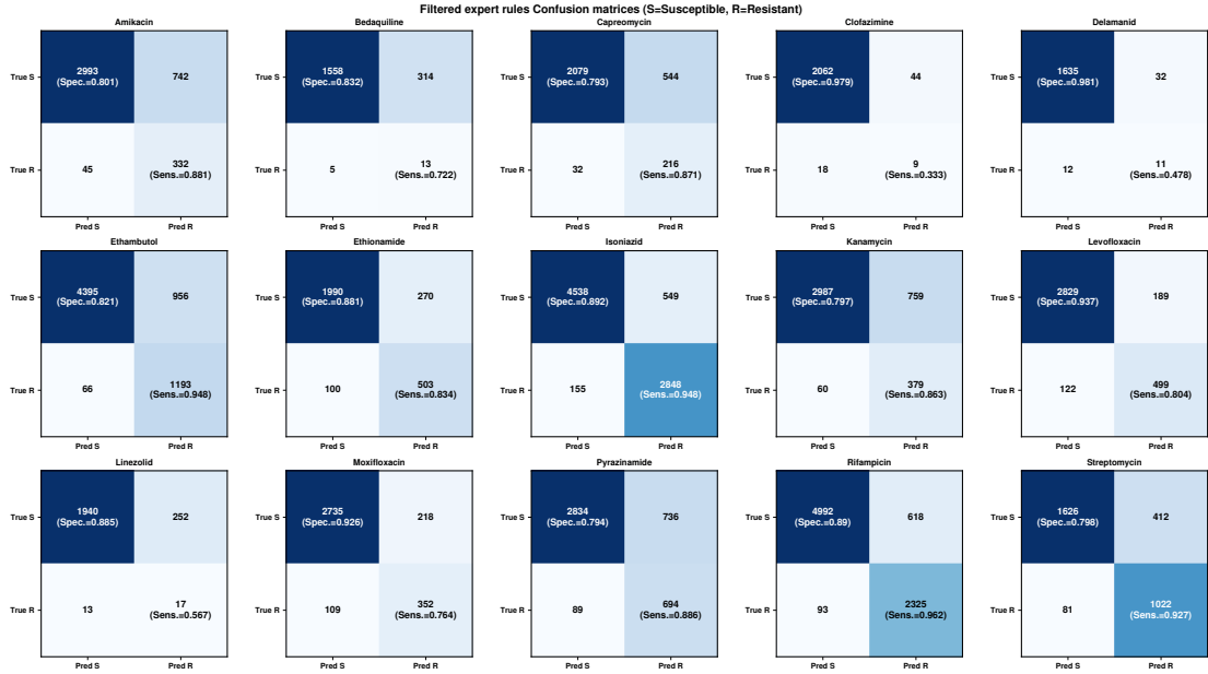
Figure 14: Confusion matrix for er+who+filt catalogue.
