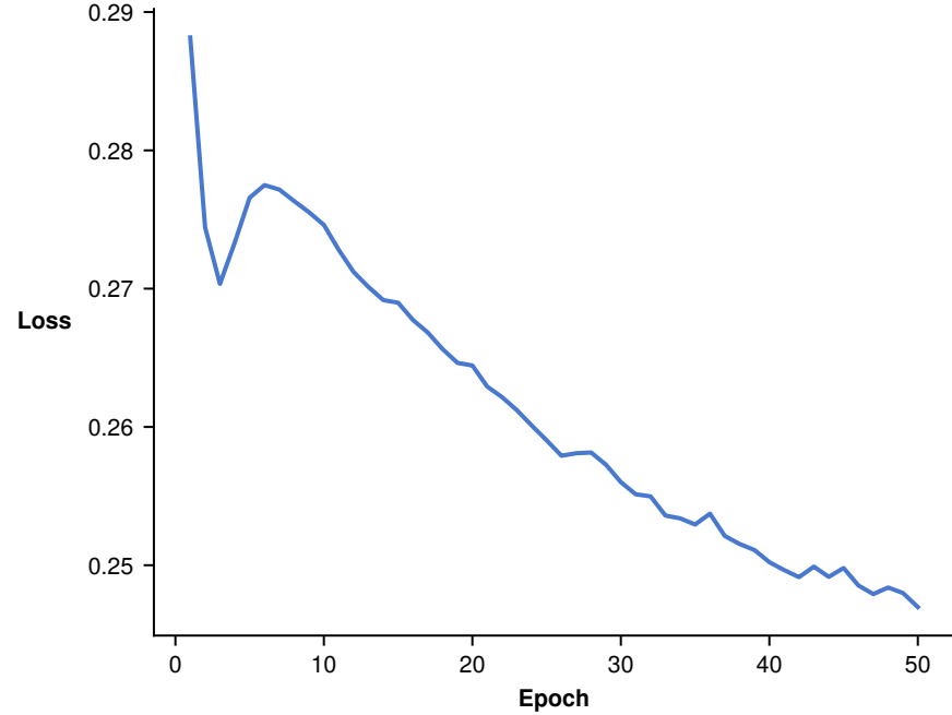
Val Loss
