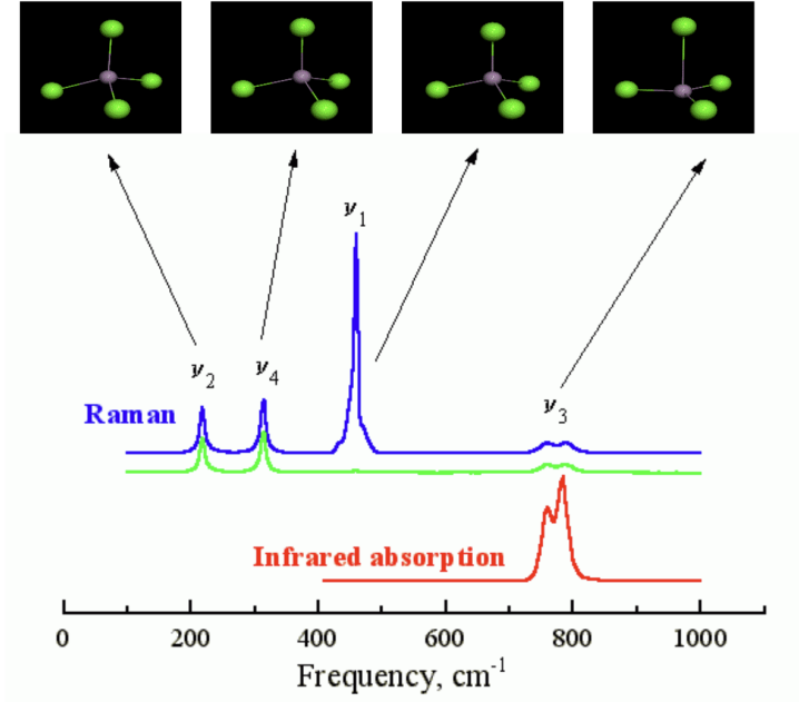
Figure 32: Raman peaks corresponding to vibrational modes. Adapted from [6]
