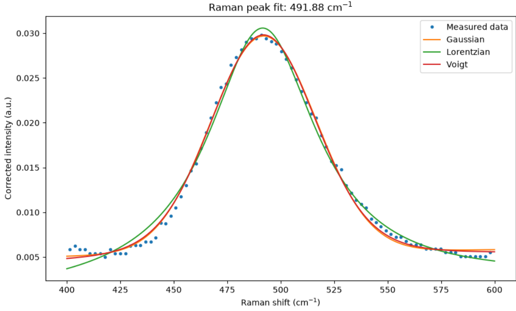
Figure 27: Fit for Raman peak at 491.9 \text{ cm}^{-1}
