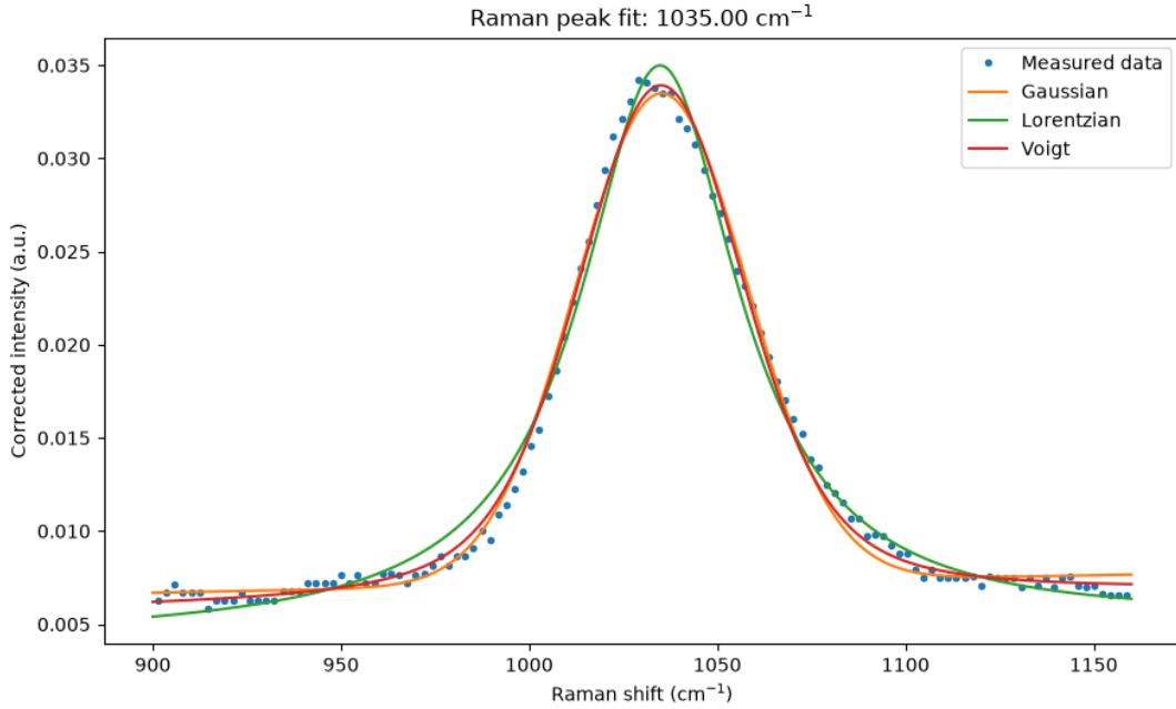
Figure 29: Fit for Raman peak at 1035 \text{ cm}^{-1}
