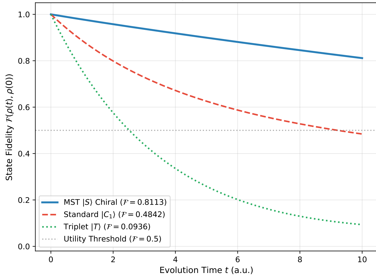
(a) Lindblad Fidelity Evolution under Mixed Bath
