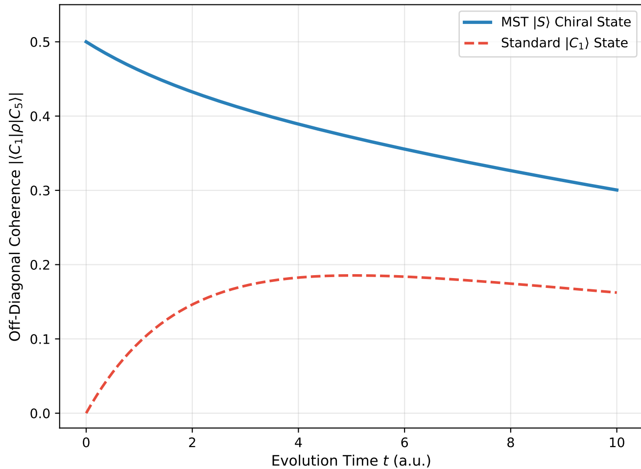
(b) Chiral Coherence Protection
