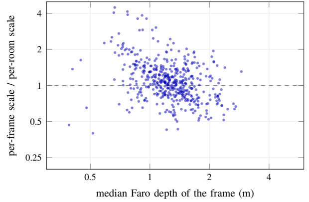
Fig. 4. Relative model DA-v2 Large, every fifth frame of the six test rooms: the per-frame oracle scale divided by the once-per-room scale, against the median Faro depth of the frame (469 frames; two frames whose fit gave no positive scale are left out). Pearson correlation of the logarithms: -0.37 .
