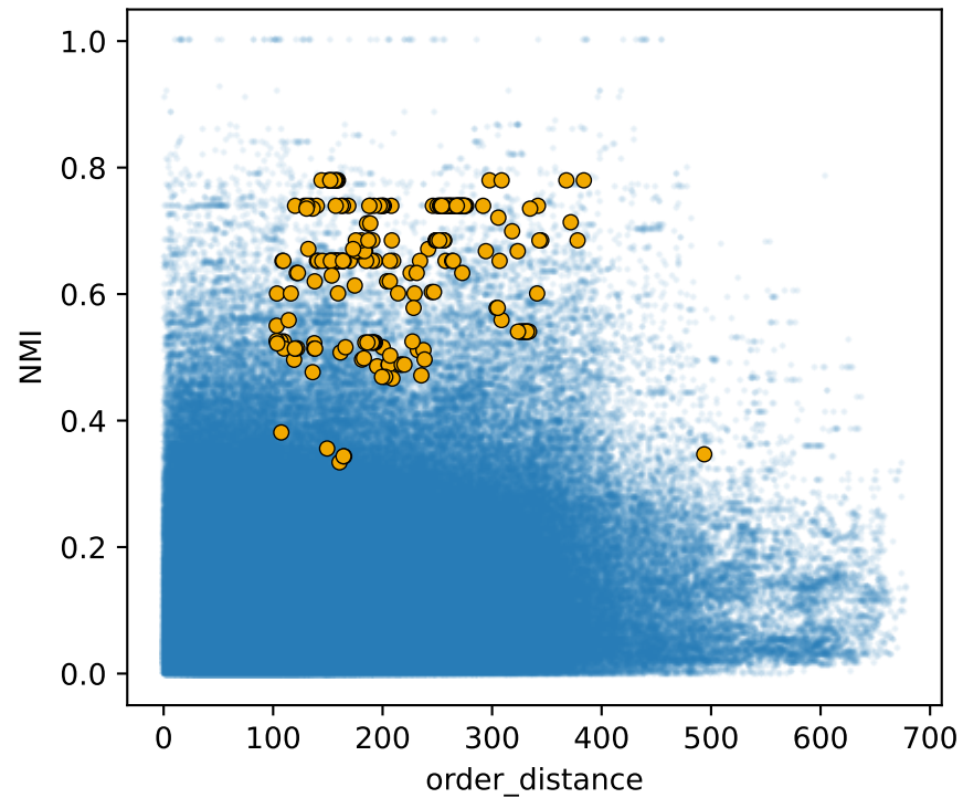
P↔T N=3,290,443
