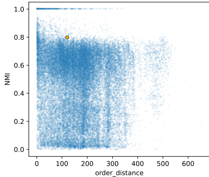
TT N=67,853
