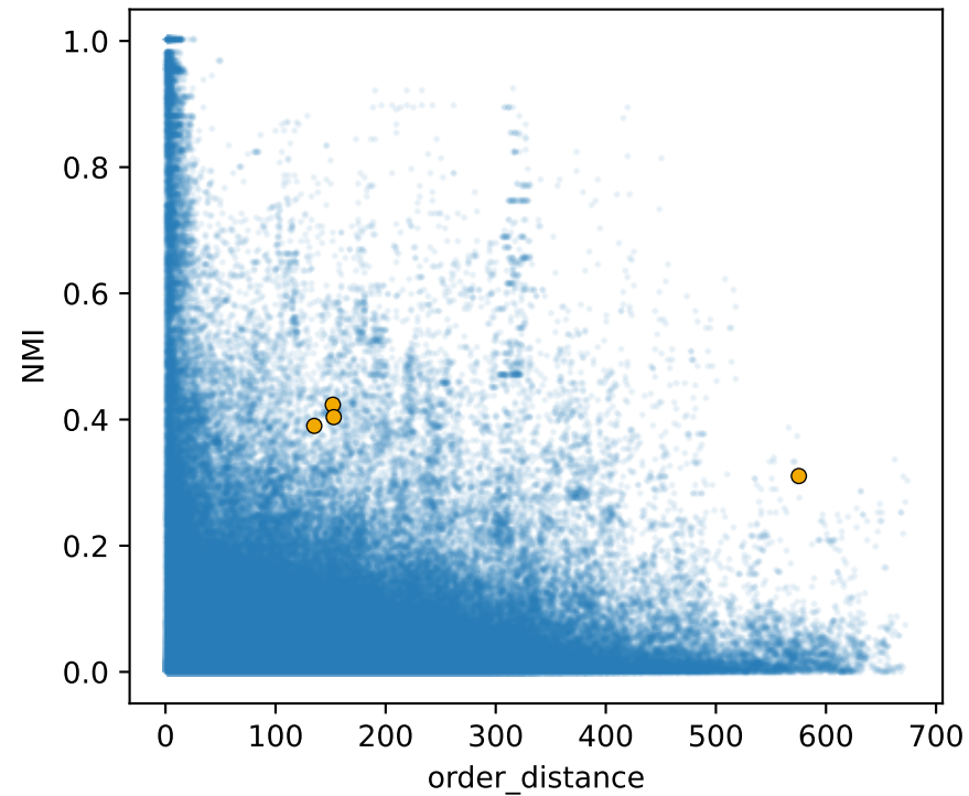
PP N=2,902,845
