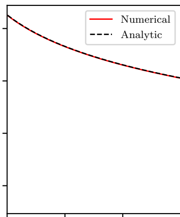
Coherent Error
