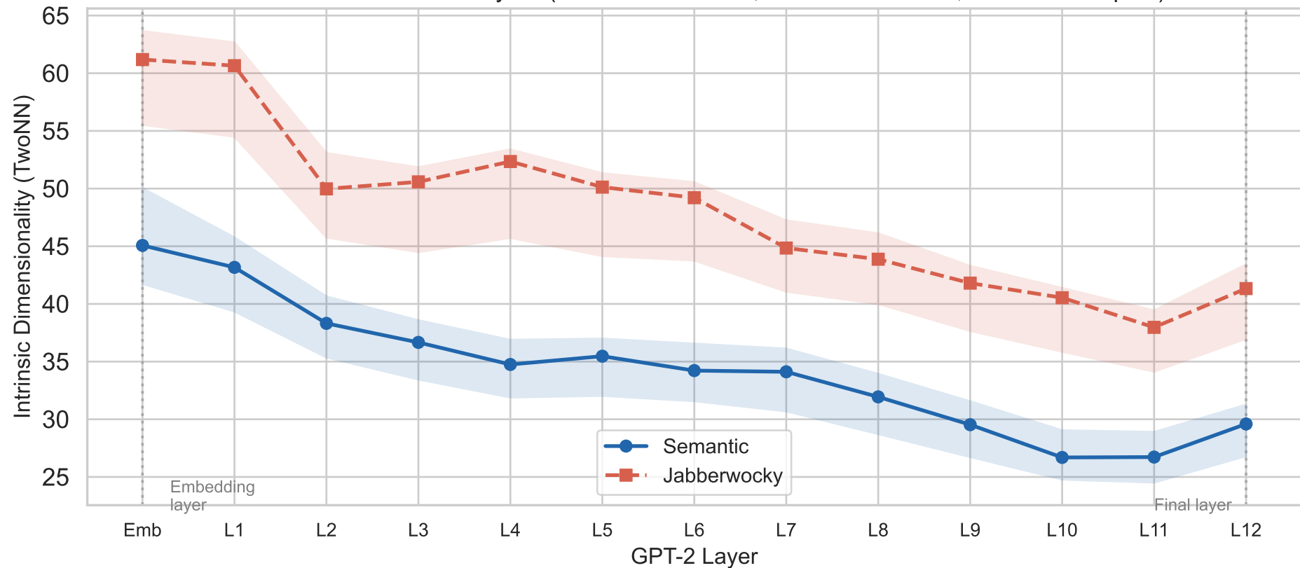
Figure 1.2 — Hunchback Profile (Mean Token Representation): ID across GPT-2 Small layers (mean of all tokens, N=500 sentences, 95% bootstrap CI)
