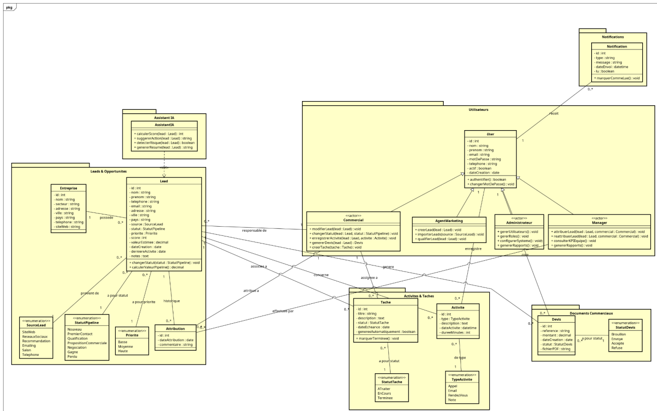
Figure 5 — Diagramme de classes du Tracking Lead System
