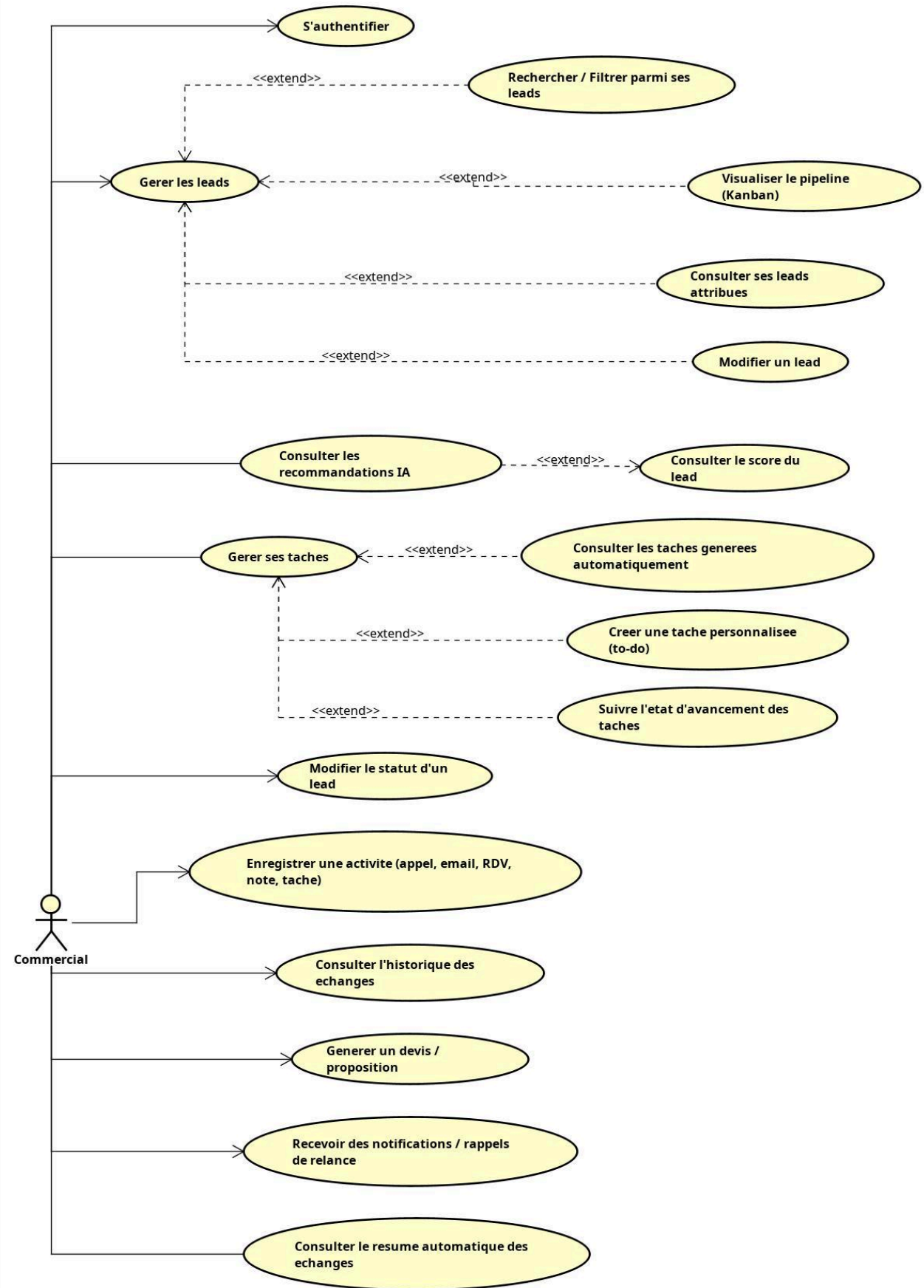
ucUseCaseDiagram_002
