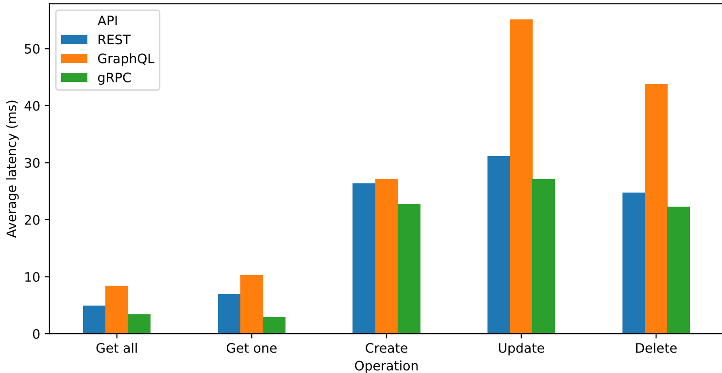
Average latency by API paradigm
