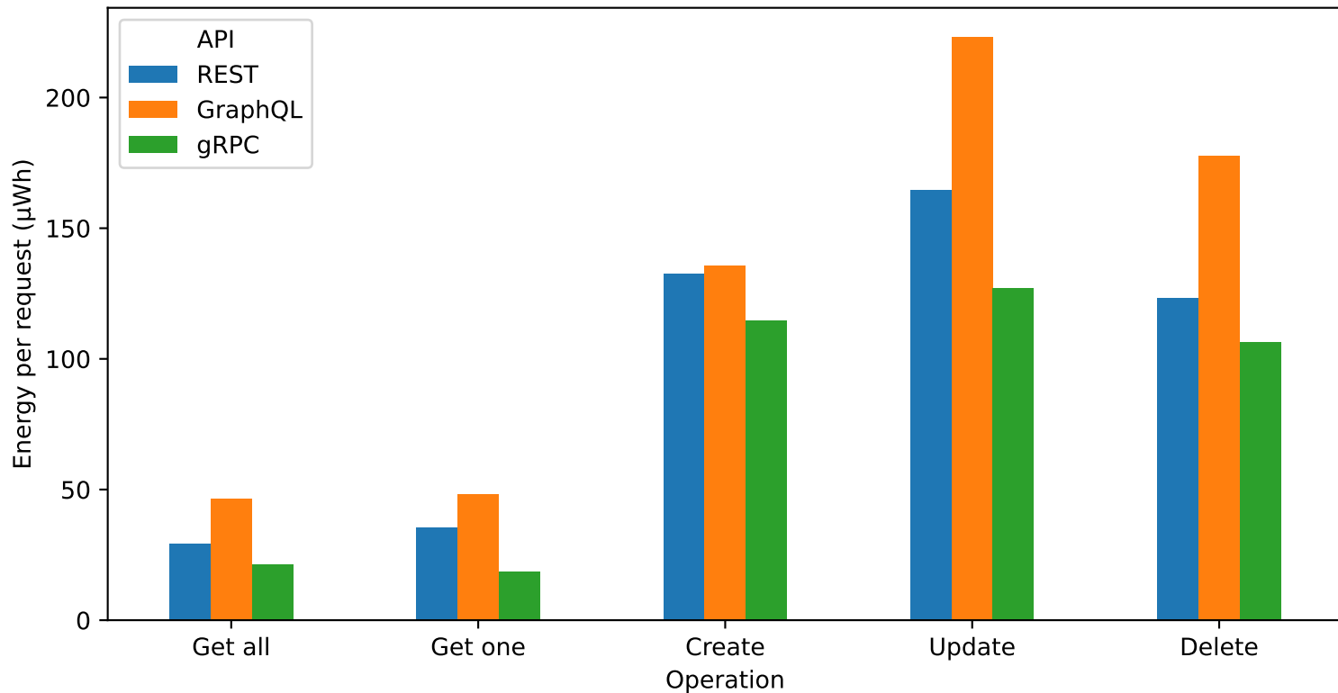
Estimated energy per request by API paradigm
