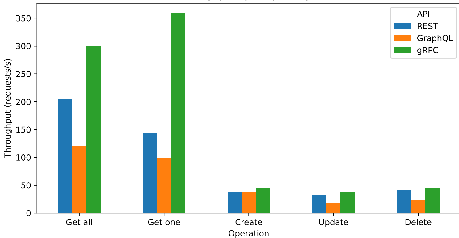
Throughput by API paradigm
