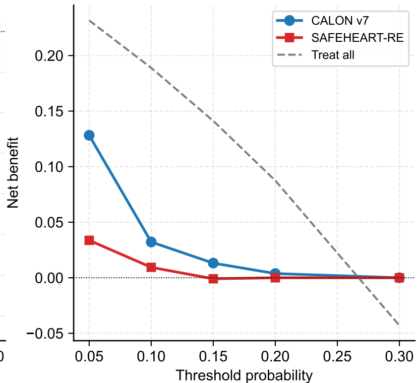
B: UKB→Wales
