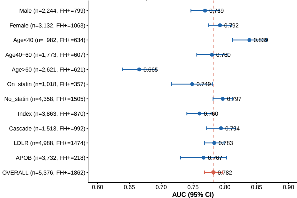
Figure 6. Subgroup-Specific TUDOR Discrimination
