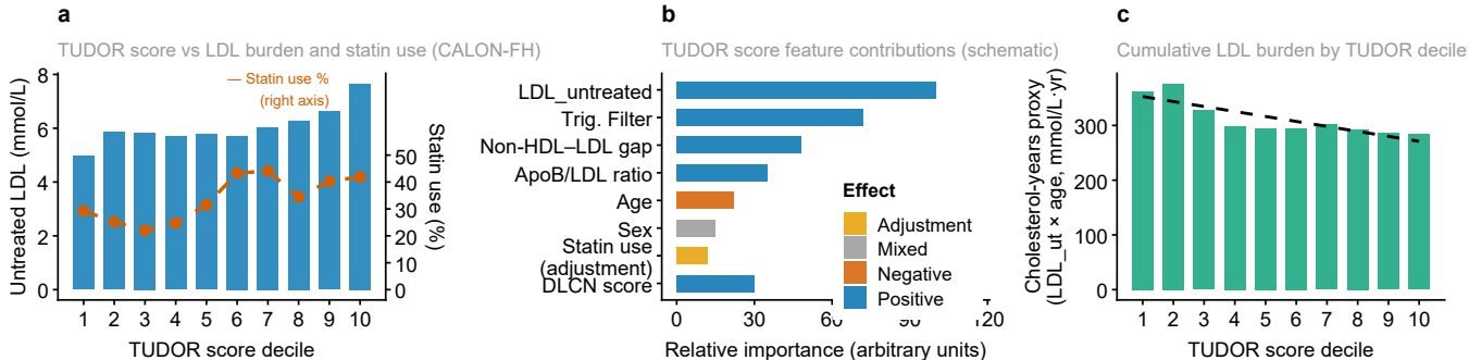
Figure 5 | TUDOR score architecture and penetrance gradient.
