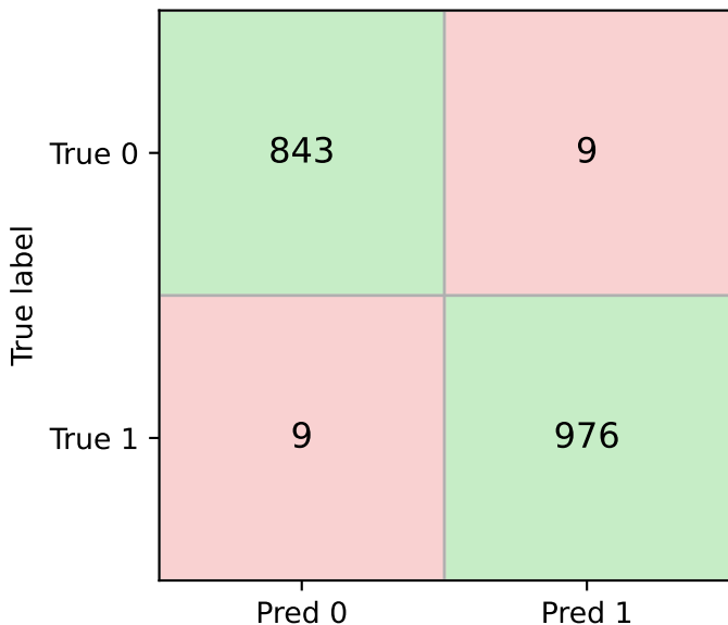
Confusion matrix (Model B, validation)
