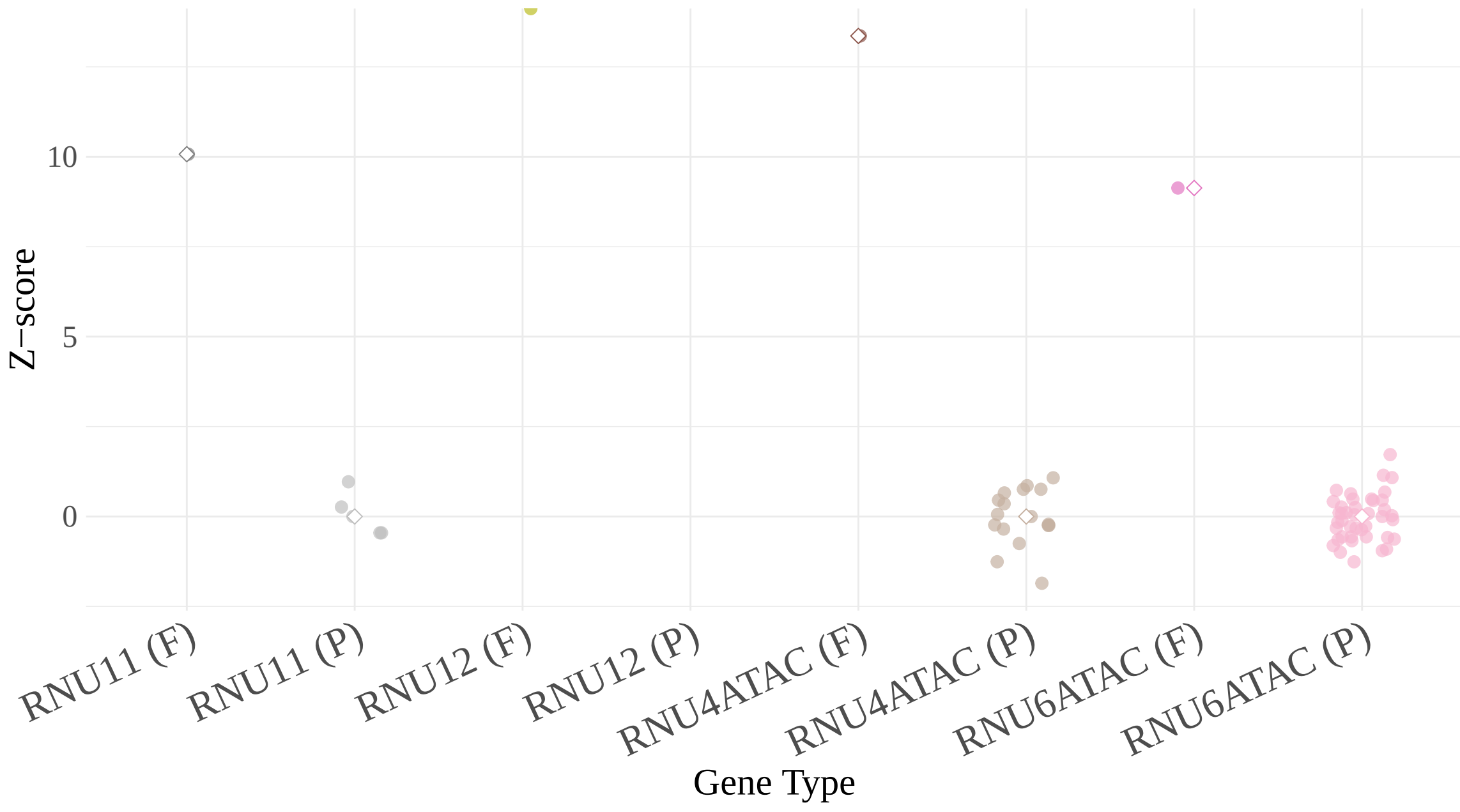
SNP Density Z-scores of Minor Spliceosomal RNAs – dbsnp
