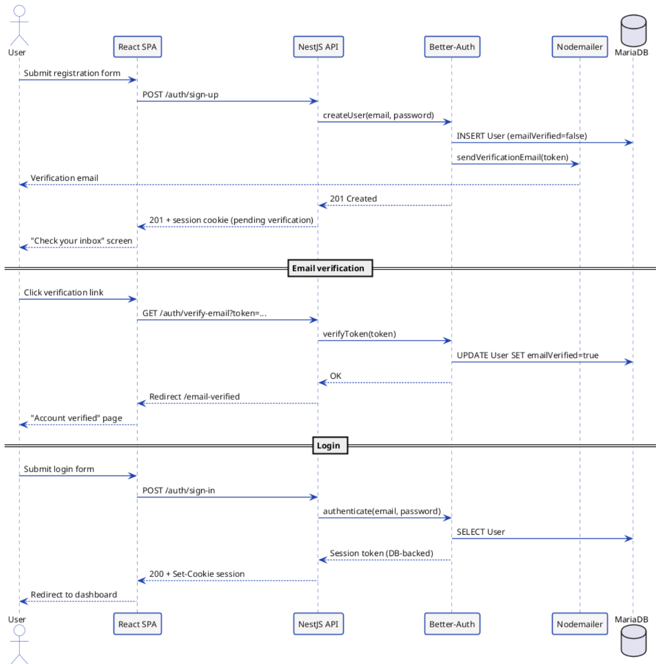
Figure 3.5: Sequence diagram — registration, email verification and login.
