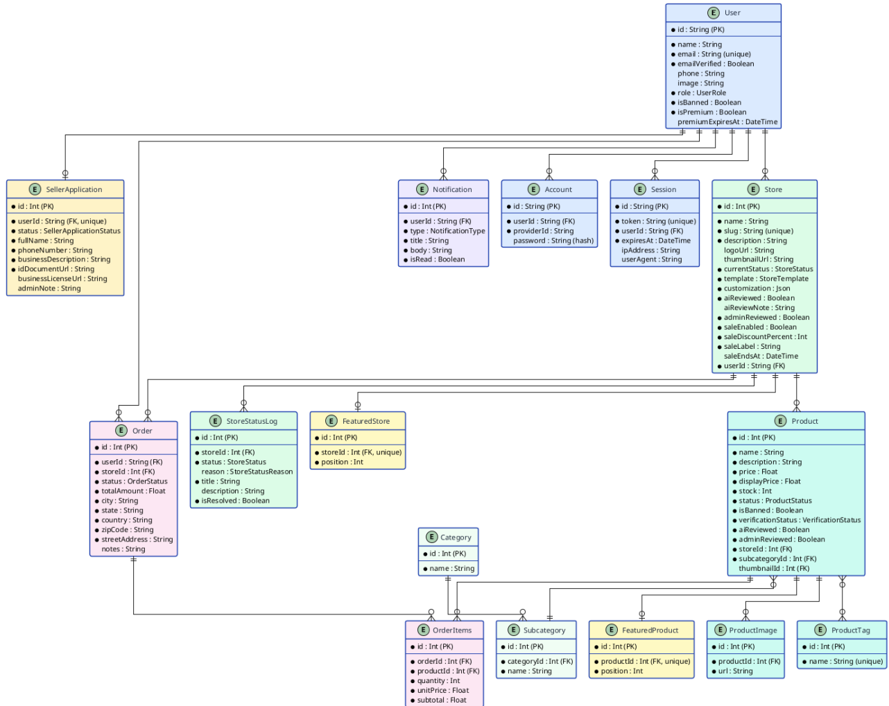
Figure 2.6: Entity-relationship diagram of the database
