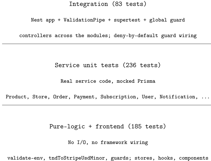
Figure 4.24: Test pyramid — 504 tests across backend (Jest, 362) and frontend (Vitest, 142).
