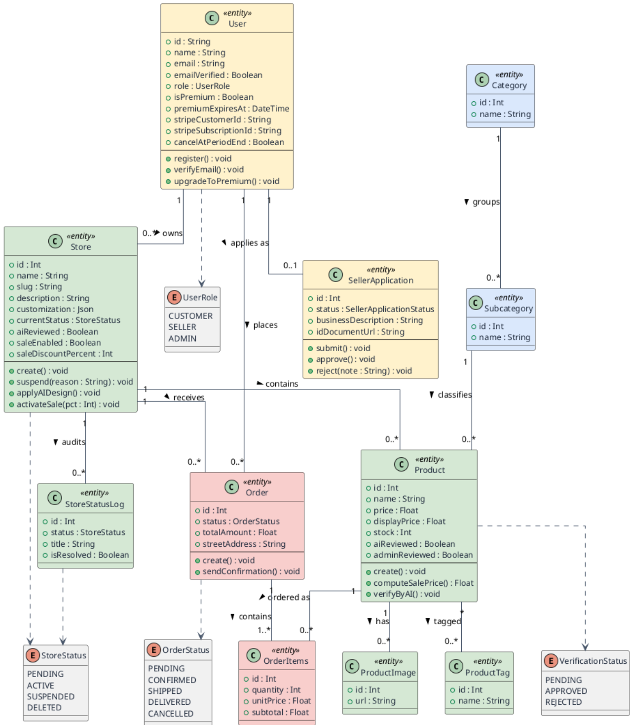
Figure 2.6: Class diagram underpinning the database schema
