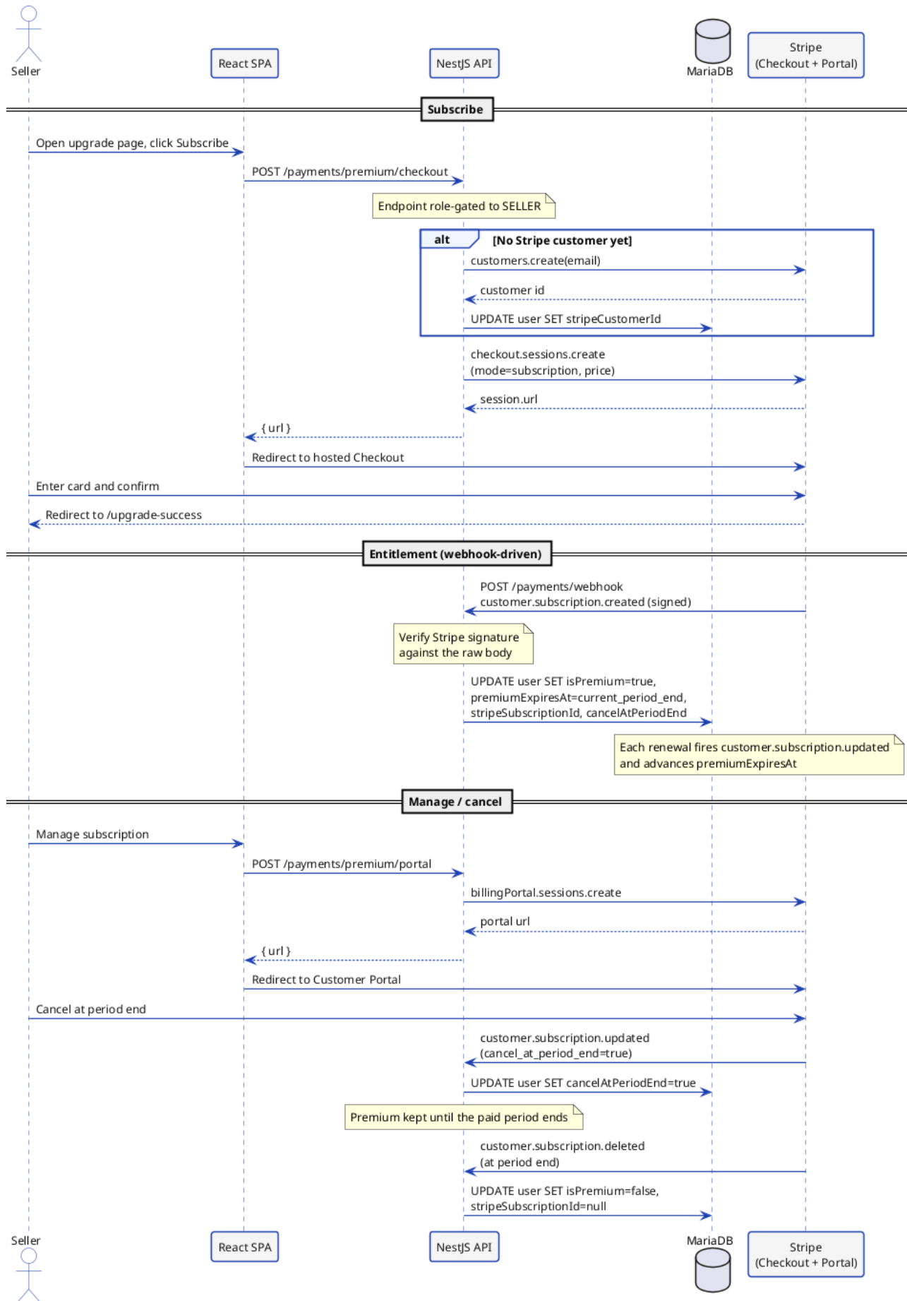
Figure 4.19: Sequence diagram — premium subscription checkout and webhook-driven entitlement.
