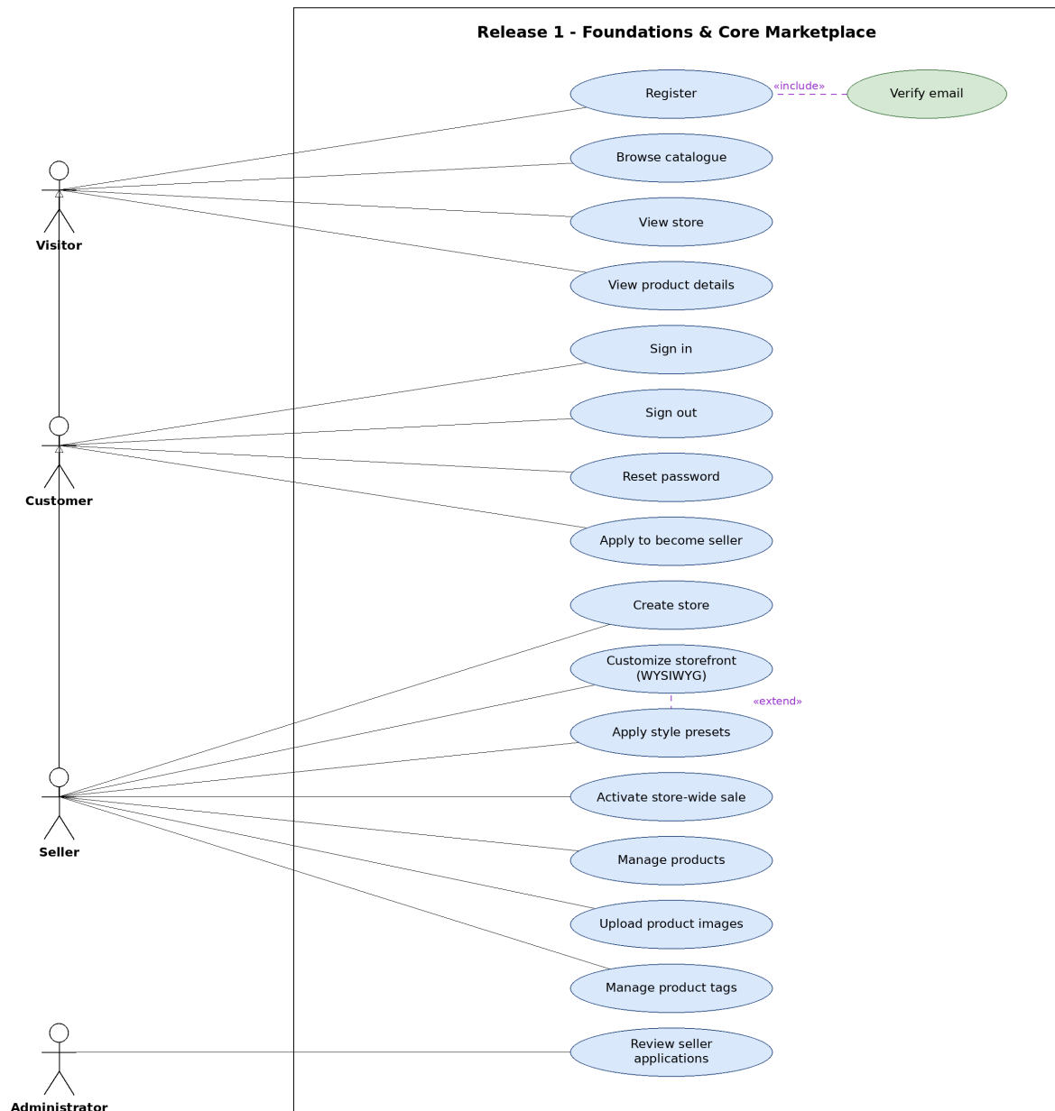
Figure 3.1: Release 1 use-case diagram (foundations and core marketplace).
