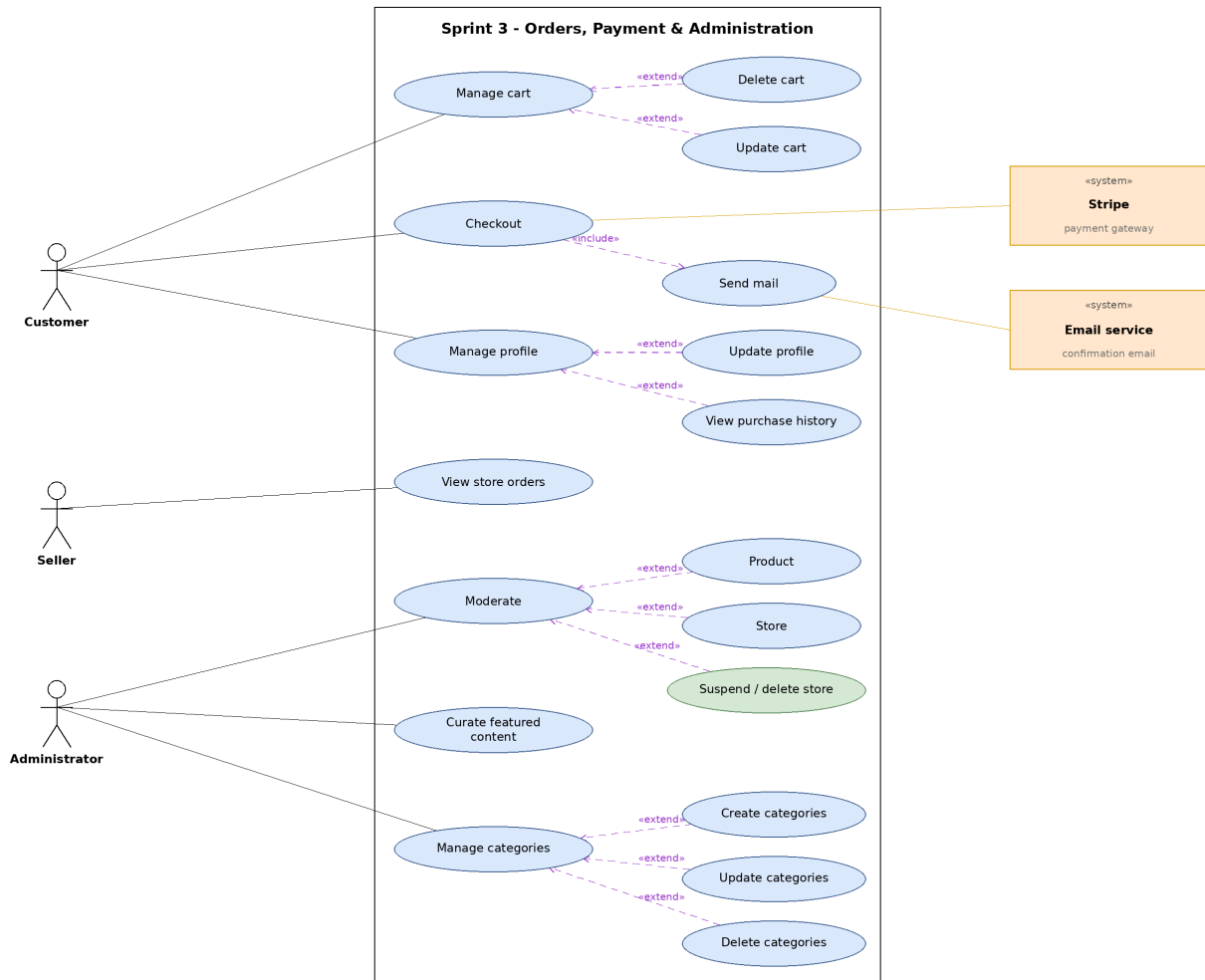
Figure 4.3: Sprint 3 use-case diagram (orders, payment and administration).
