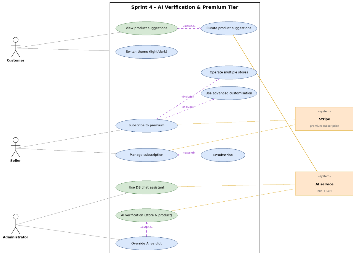
Figure 4.12: Sprint 4 use-case diagram (AI verification and premium tier).
