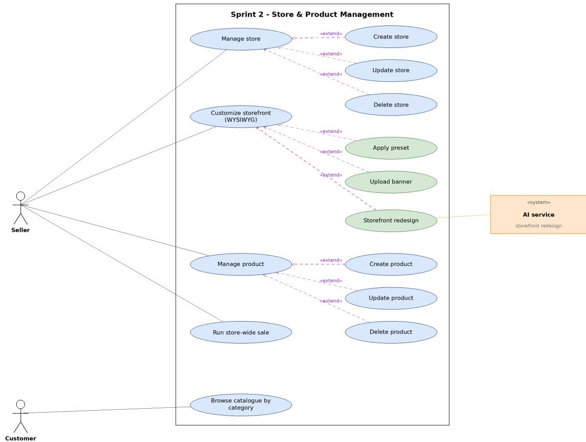
Figure 3.12: Sprint 2 use-case diagram (store and product management).
