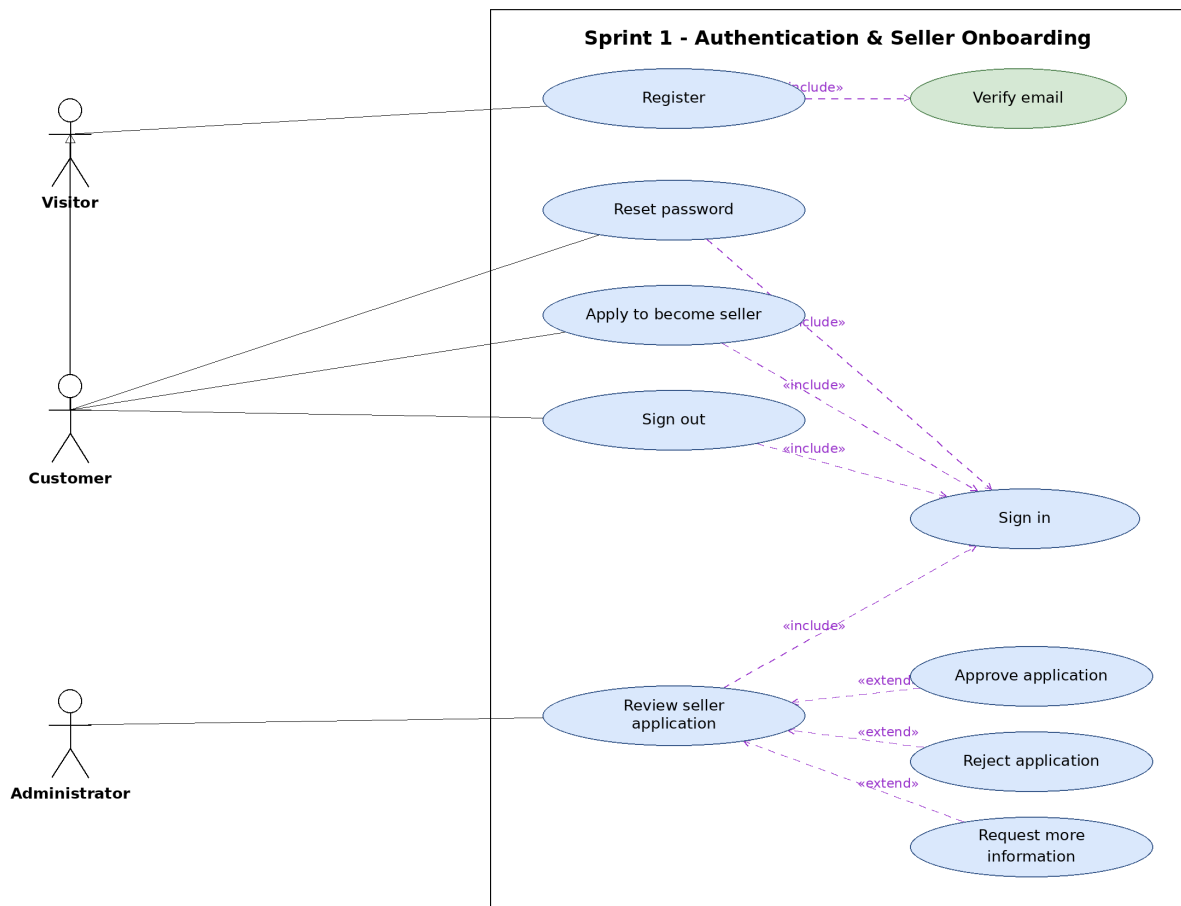
Figure 3.3: Sprint 1 use-case diagram (authentication and seller onboarding).
