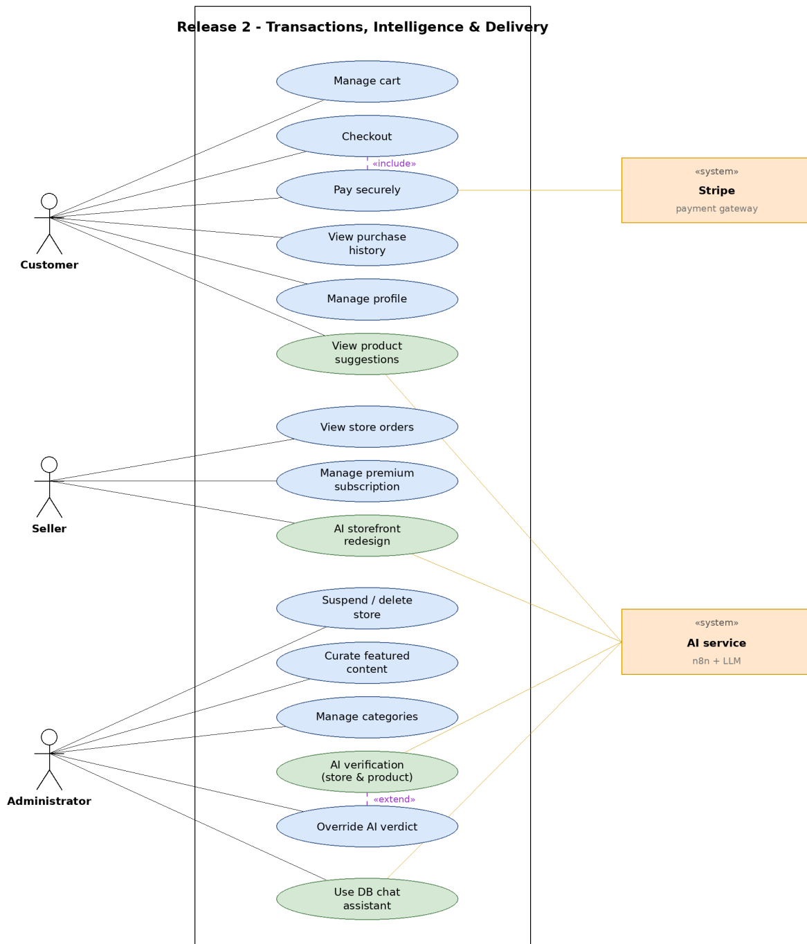
Figure 4.1: Release 2 use-case diagram (transactions, intelligence and delivery).
