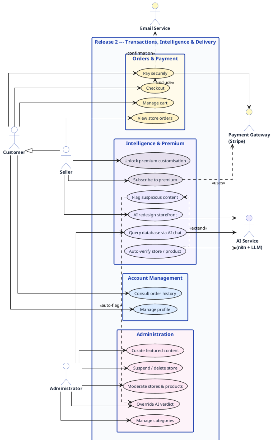
Figure 4.1: Release 2 use-case diagram (transactions, intelligence and delivery).
