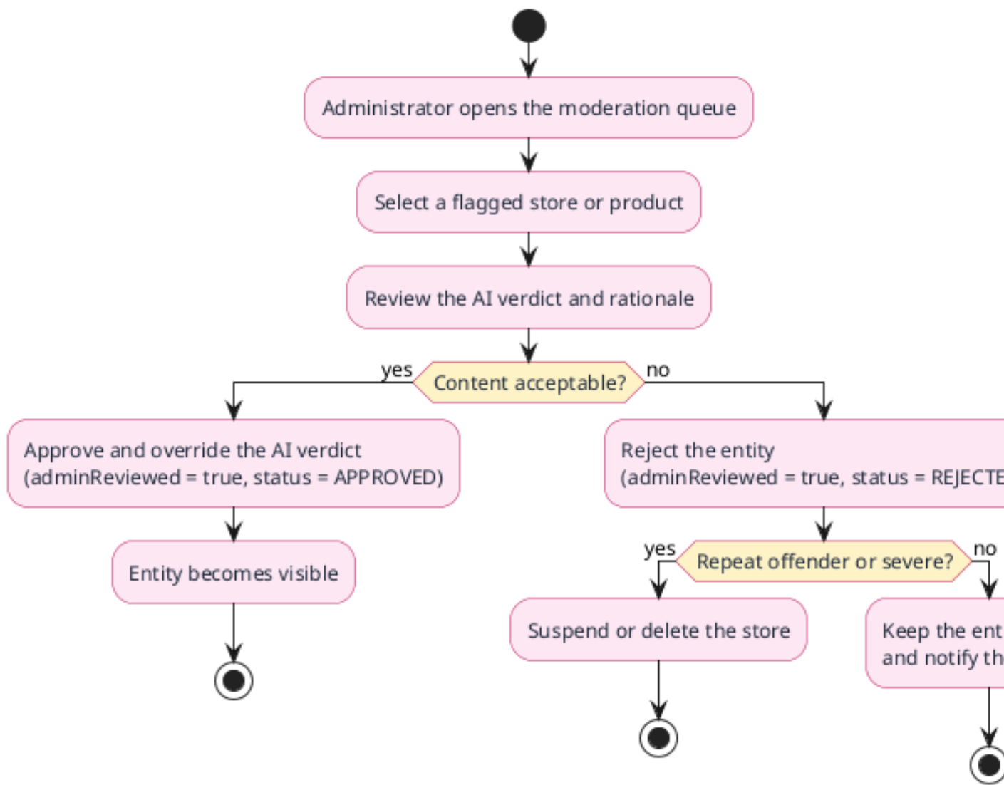
Figure 4.14: Activity diagram — content moderation.
