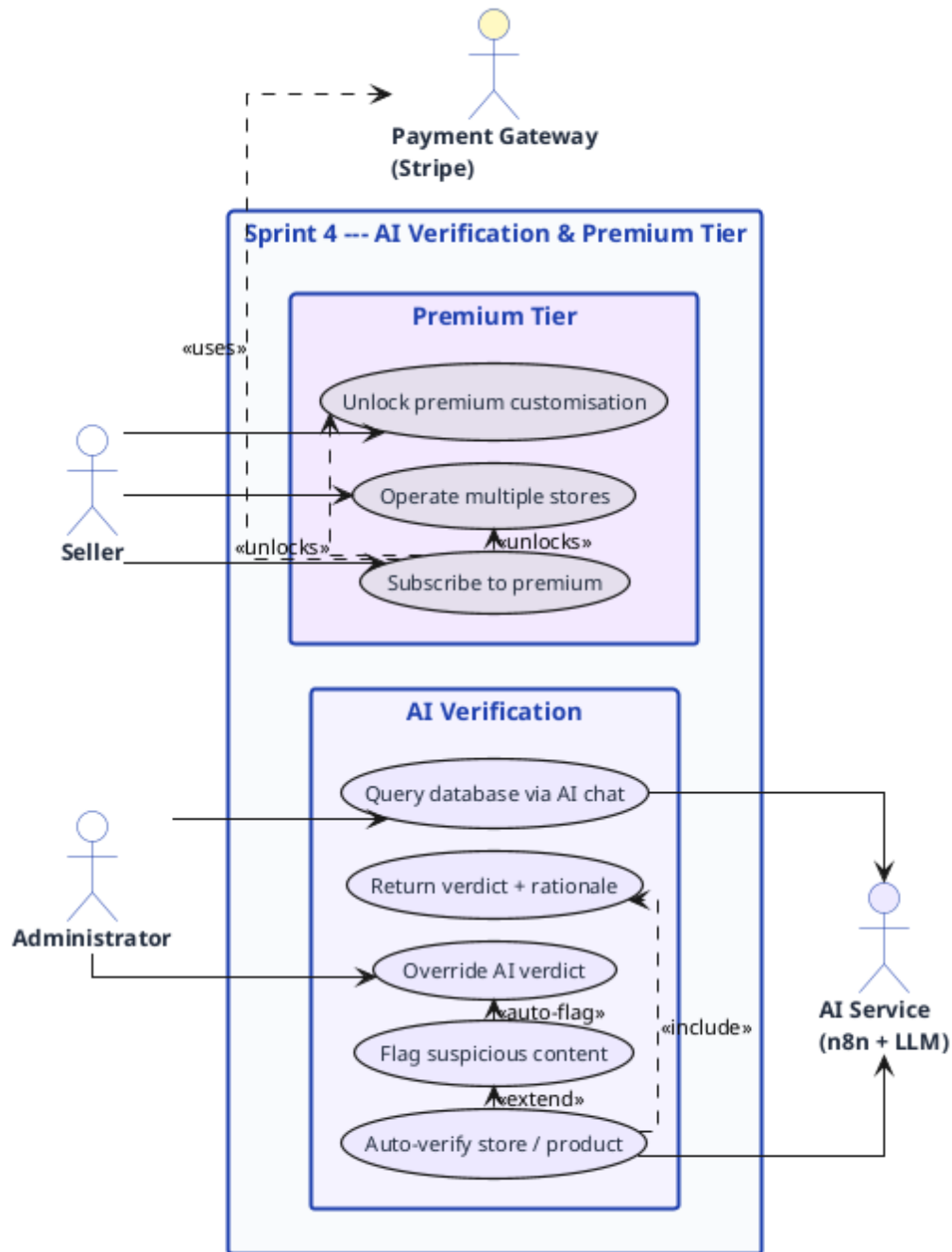
Figure 4.12: Sprint 4 use-case diagram (AI verification and premium tier).
