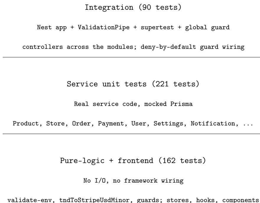
Figure 4.21: Test pyramid — 473 tests across backend (Jest, 346) and frontend (Vitest, 127).
