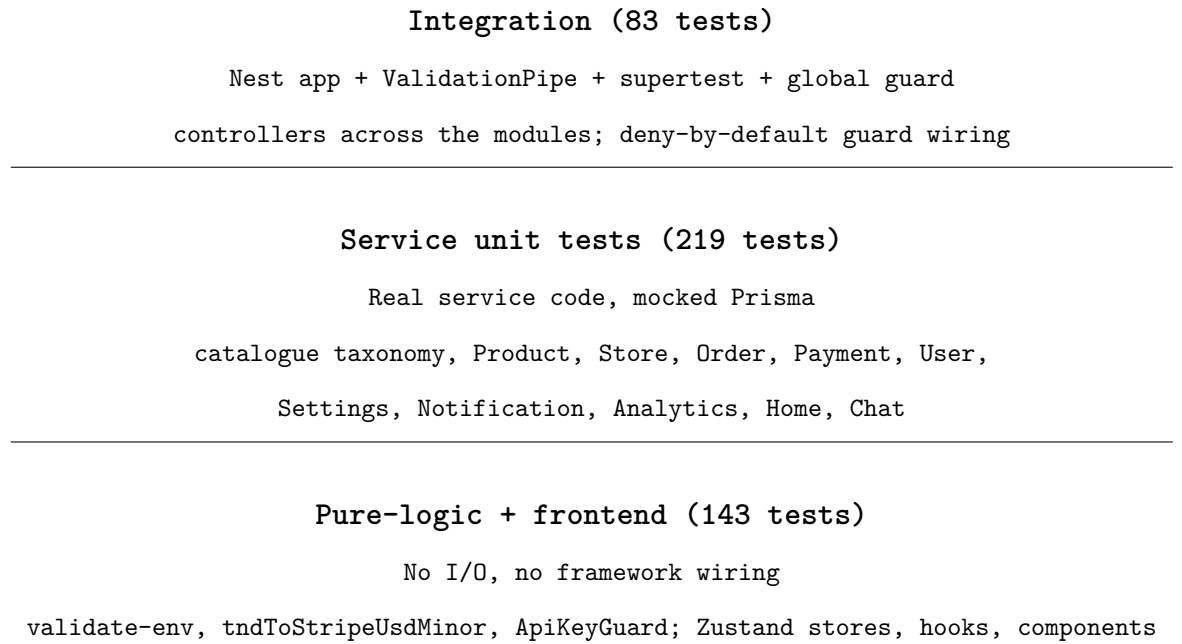
Figure 4.25: Test pyramid — 445 tests total across backend (Jest, 337) and frontend (Vitest, 108)
