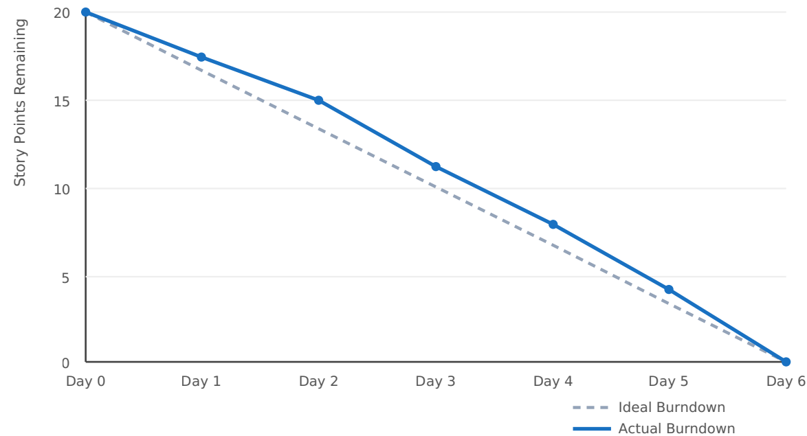
Figure 1: Sprint-1 burndown chart - story points remaining vs. time, comparing ideal and actual progress
