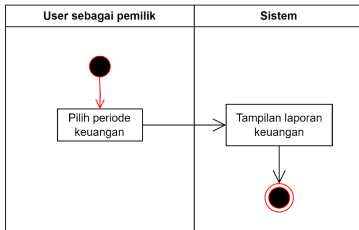
Gambar 3. 20 Activity Diagram proses menerima laporan
