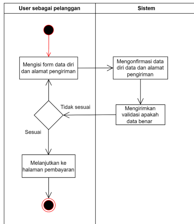
Gambar 3. 16 Activity Diagram proses mengisi form pengiriman
