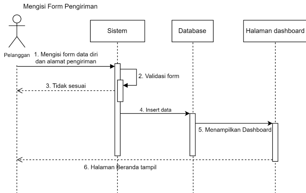
Gambar 3. 8 Sequence Diagram Mengisi Form Pengiriman
