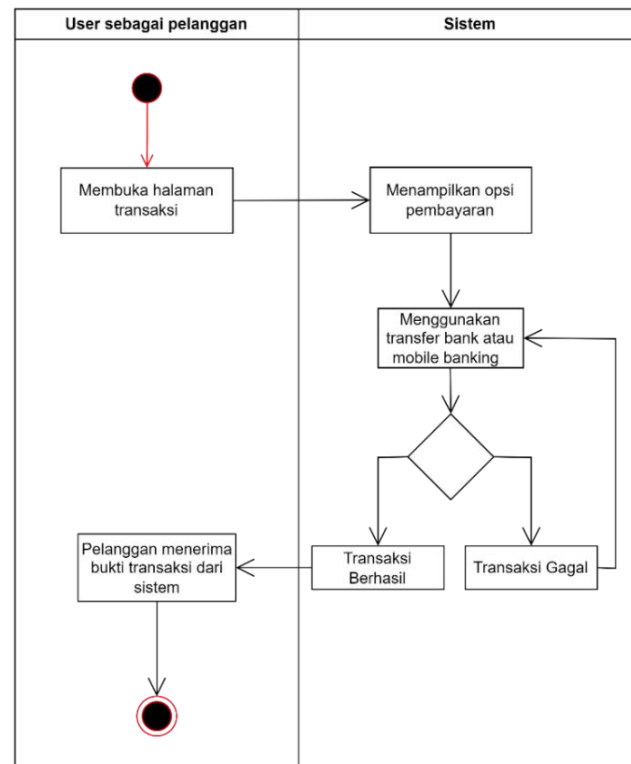
Gambar 3. 17 Activity Diagram proses transaksi online
