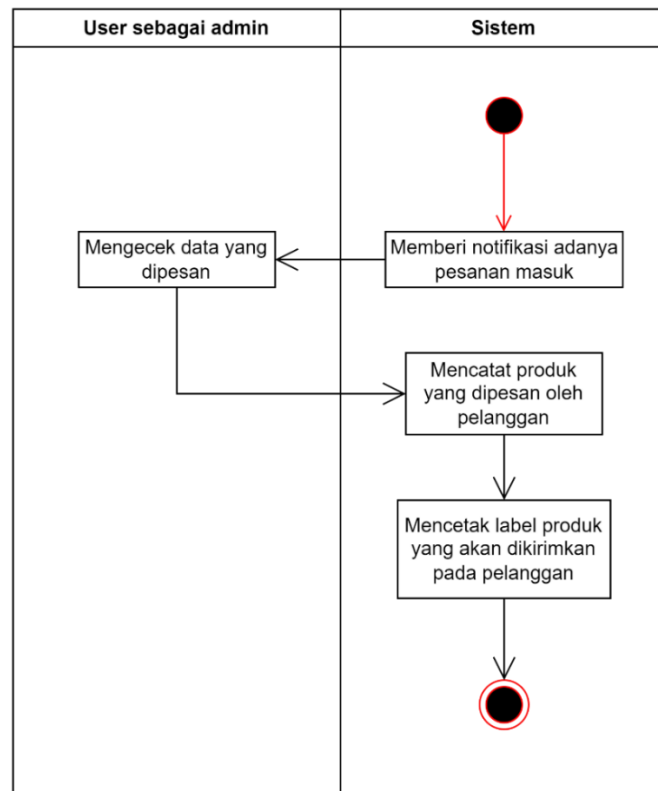
Gambar 3. 18 Activity Diagram proses mengelola data pesanan
