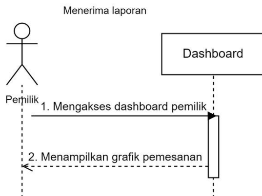
Gambar 3.12 Sequence Diagram Menerima Laporan
