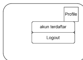
Gambar 3. 29 Interface Logut
