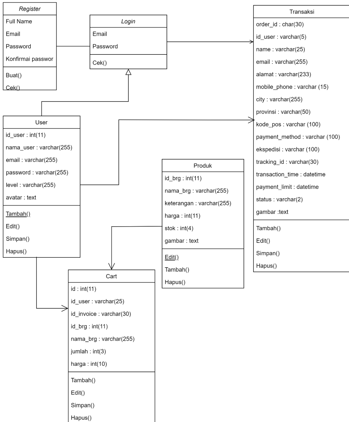
Gambar 3. 4 Class Diagram
