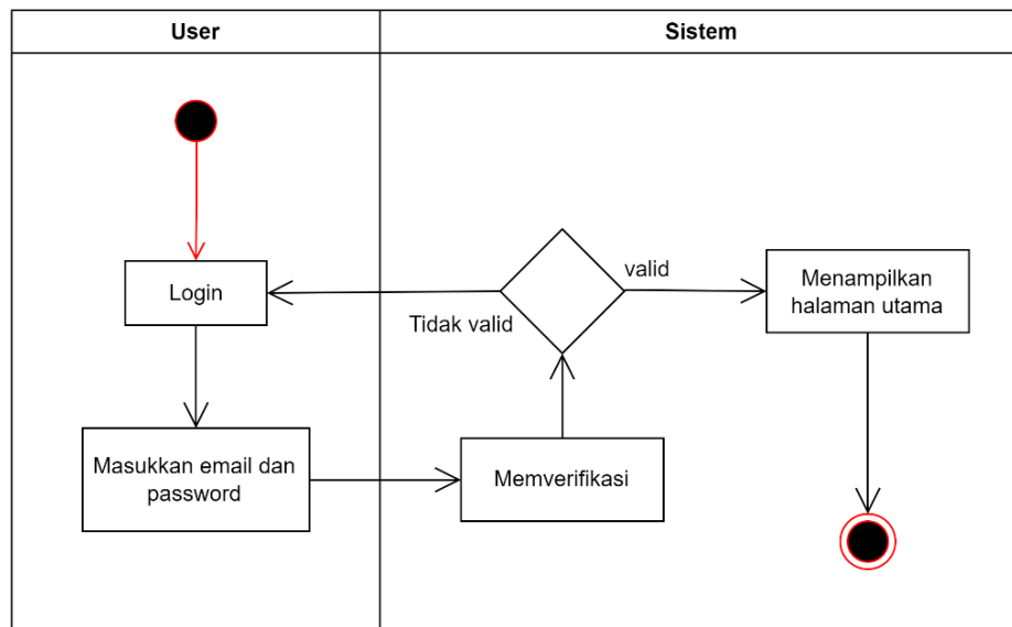
Gambar 3. 14 Activity Diagram proses login
