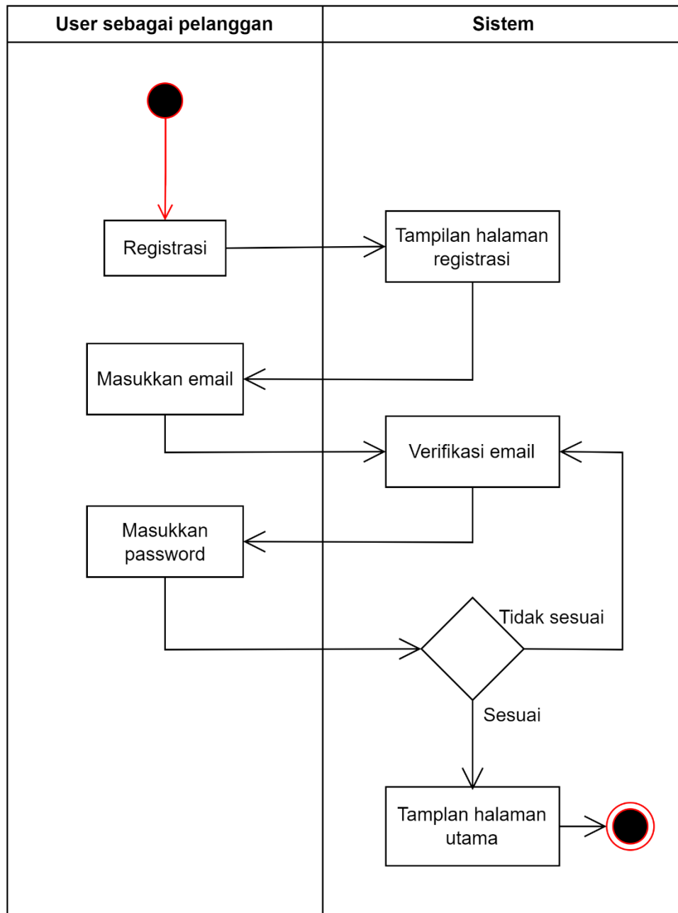
Gambar 3. 13 Activity Diagram proses registrasi
