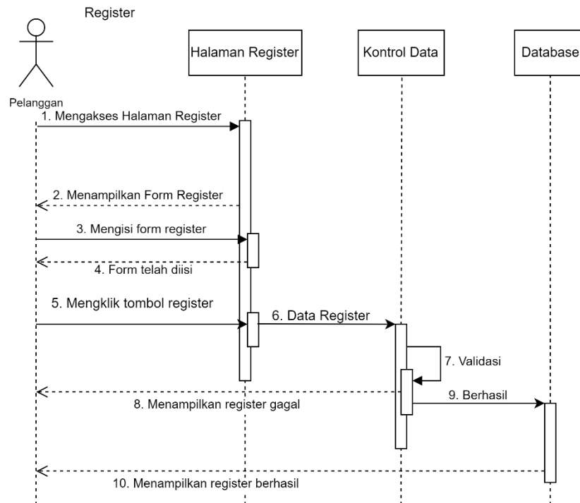
Gambar 3. 5 Sequence Diagram Registrasi
