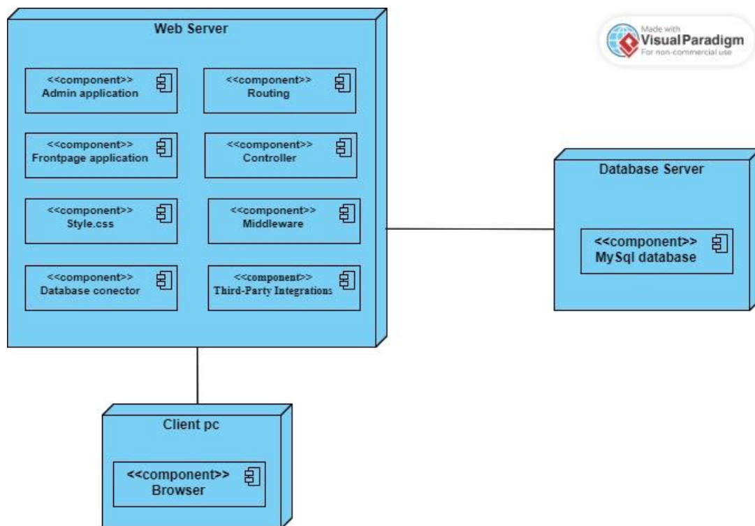
Gambar 3. 21 Deployment Diagram
