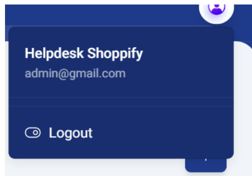
Gambar 4. 17 Tampilan Logout
