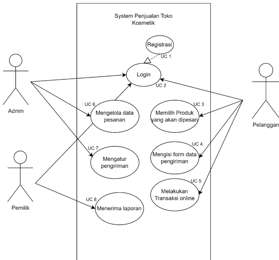
Gambar 3. 3 Usecase Diagram
