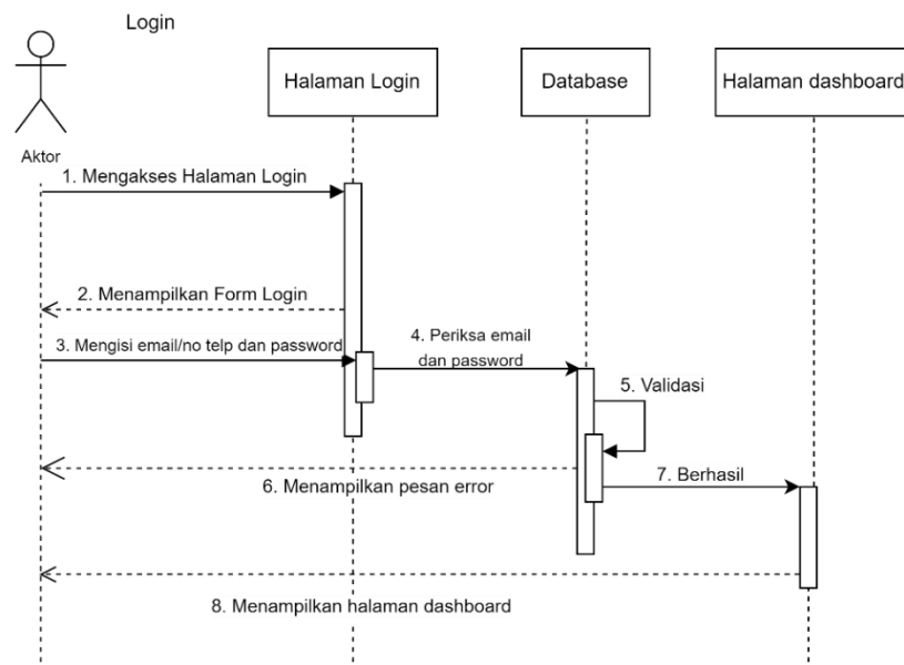
Gambar 3. 6 Sequence Diagram Login
