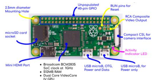
Figure 19: Raspberry Pi Zero
