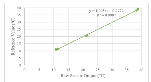
Figure 4: Calibration Curve of the Temperature Sensor
