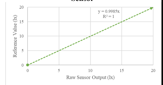
Figure 3: Calibration Curve of Light Intensity Sensor
