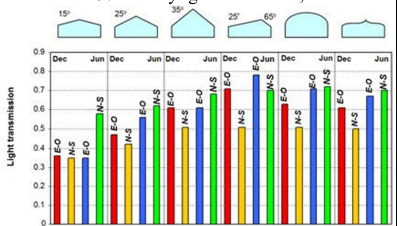
Figure 17, transmissivity for several greenhouses' geometric shape (Valera Martínez et al., 2016).
