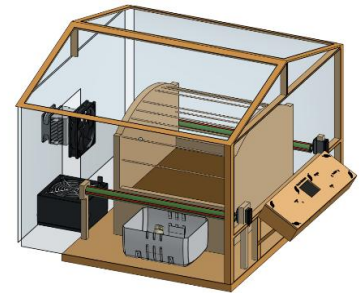
Figure 1: 3D CAD model for the prototype
