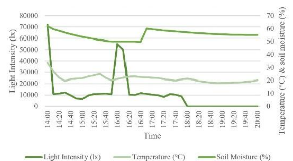
Figure 10: Temperature, Soil Moisture, and Light Intensity readings over 6 hours
