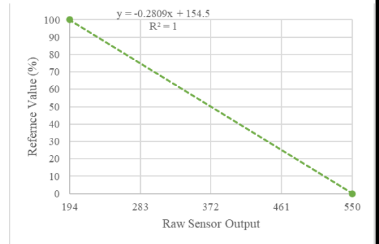
Figure 2: Calibration Curve of Soil Moisture Sensor
