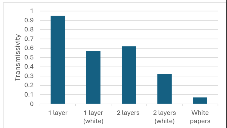
Figure 16, transmissivity for several plastic films and papers
