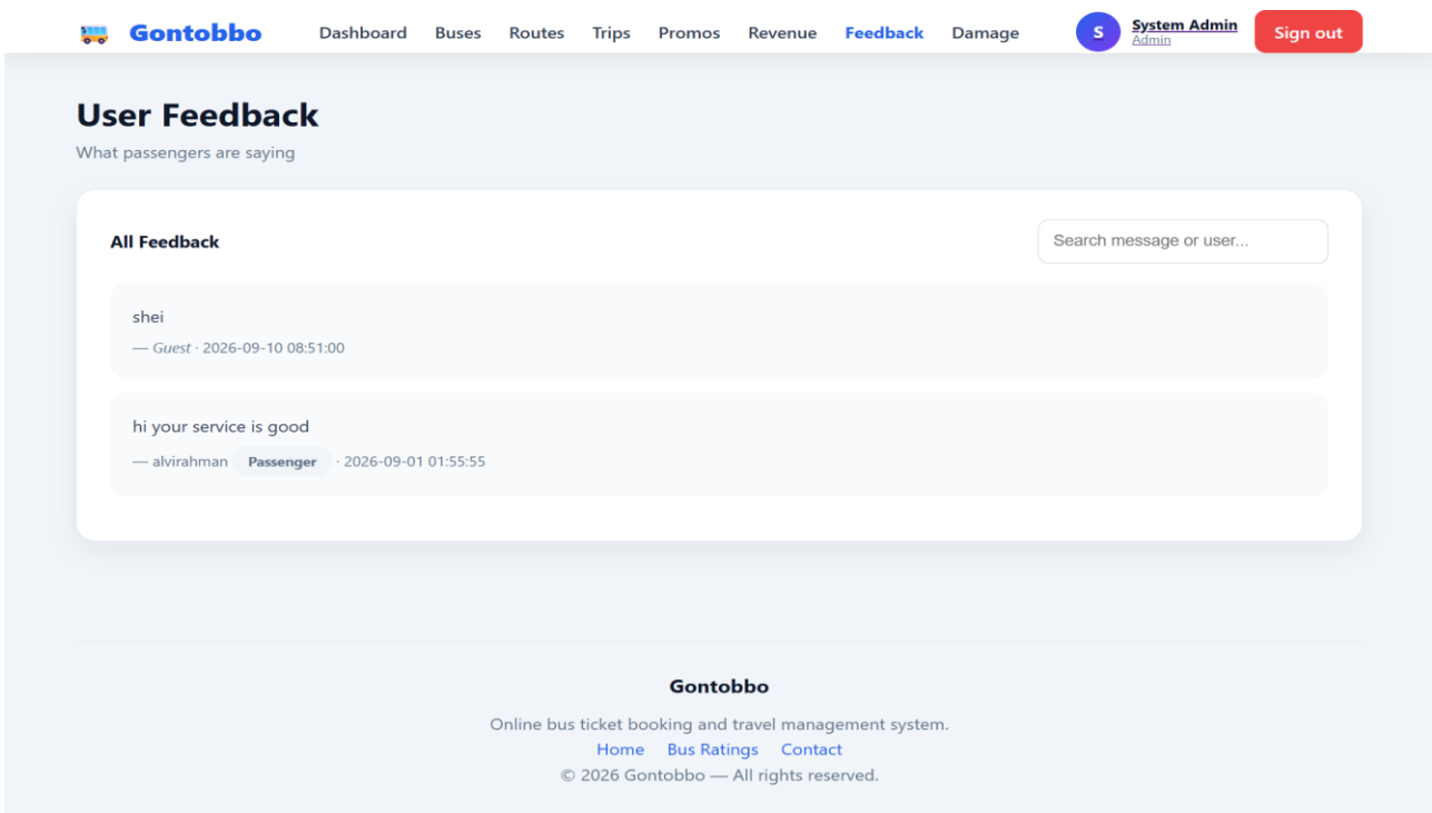
Fig 22: ADMIN — FEEDBACK
