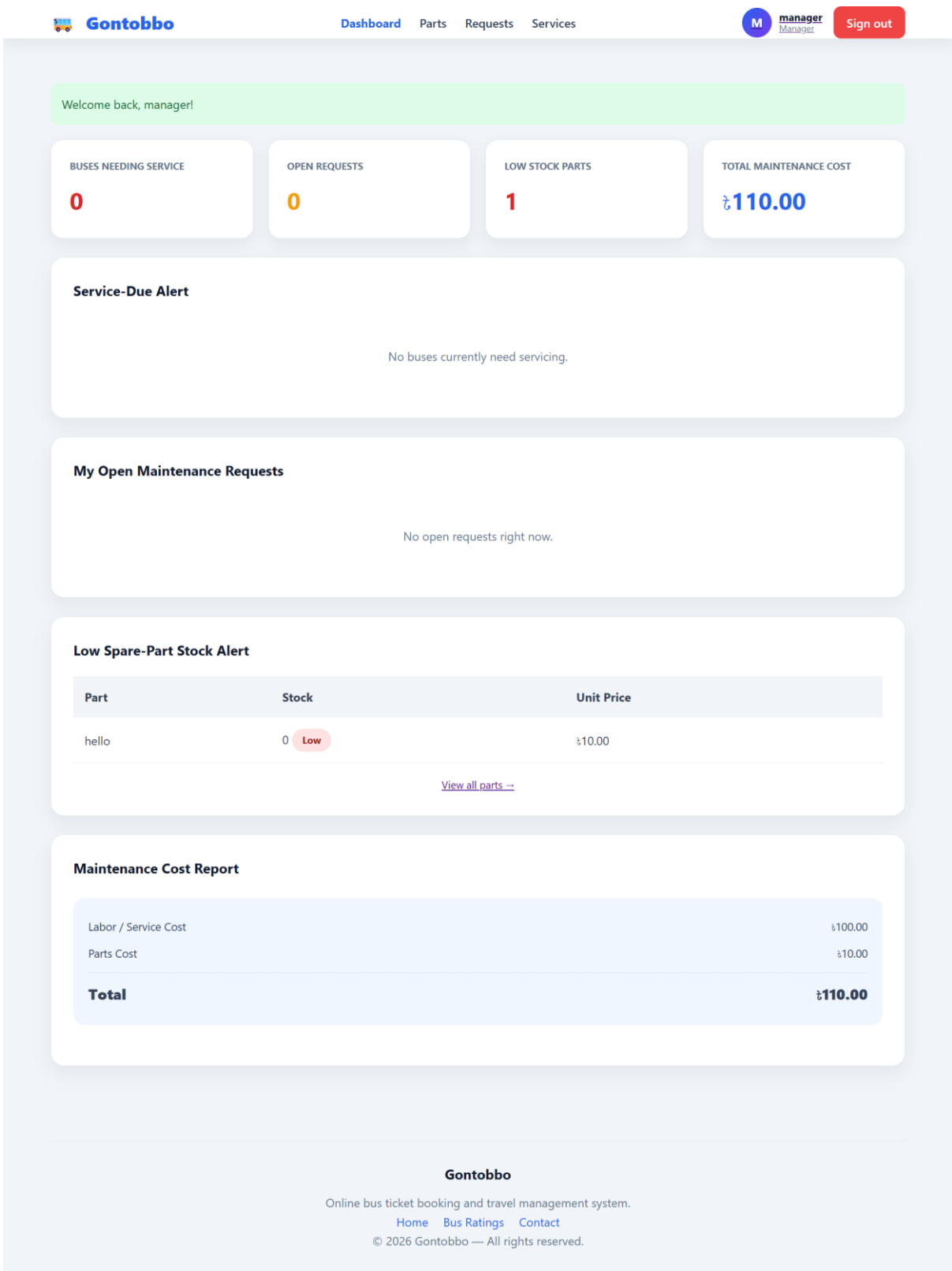
Fig 29: MANAGER — DASHBOARD
