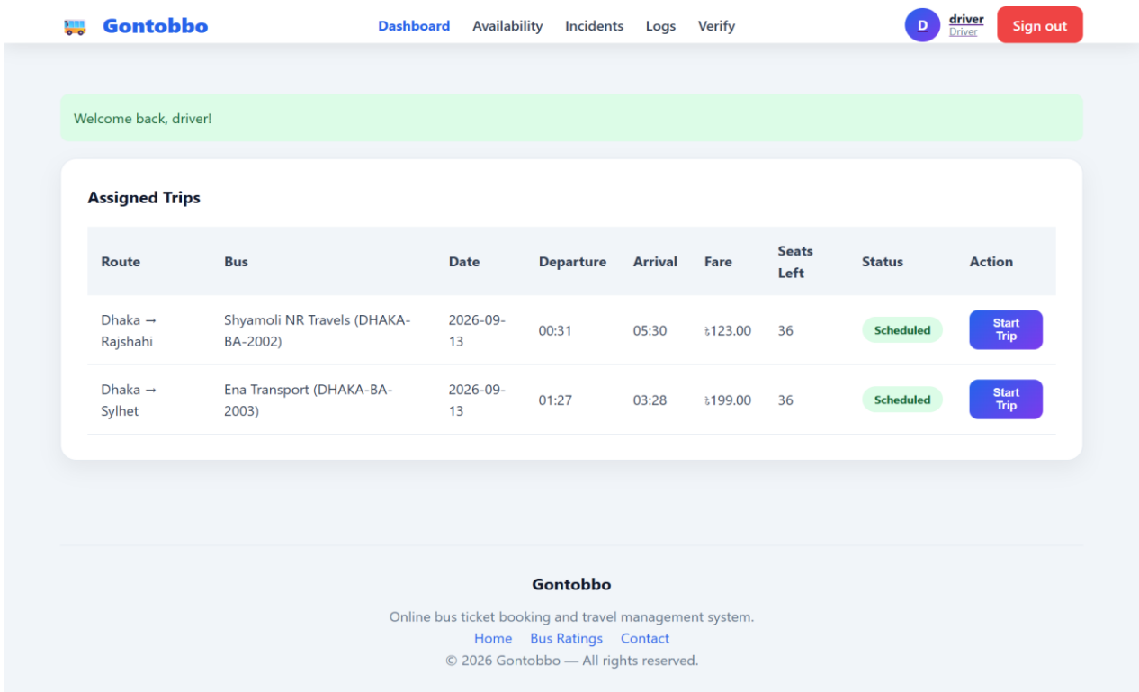
Fig 24: DRIVER — DASHBOARD
