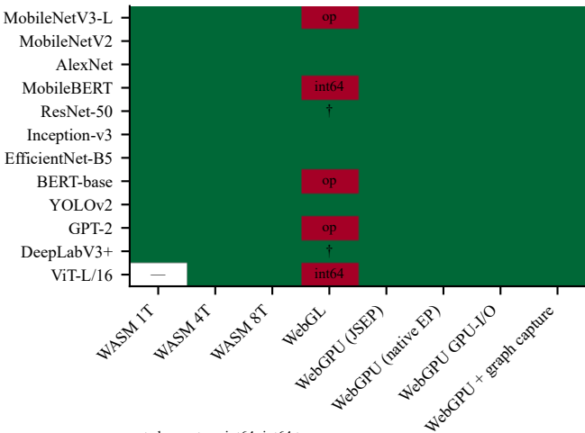
Verified execution (green) and failure cause
