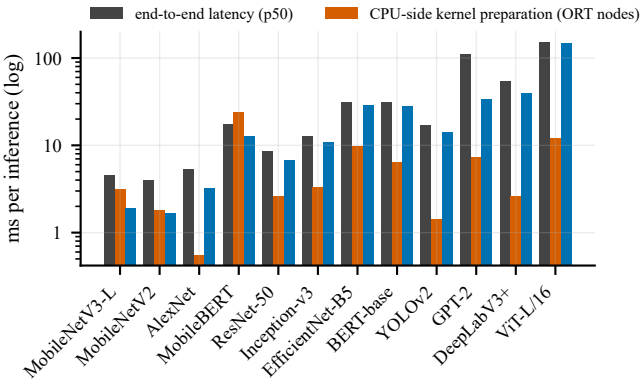
(a) WebGPU (JSEP): where one inference's time goes
