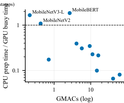
(b) >1 : the CPU, not the GPU, is the bottleneck
