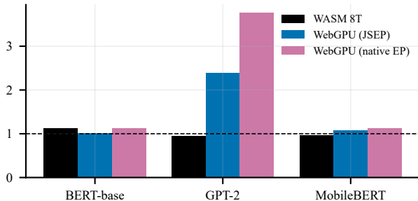
(a) Cost of fetching every output
