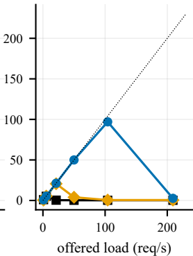
ResNet-50
