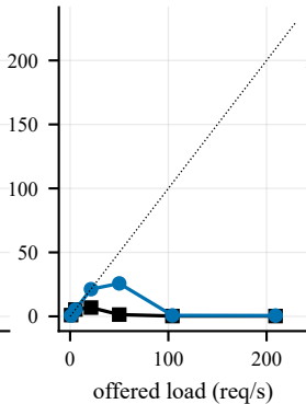
MobileBERT
