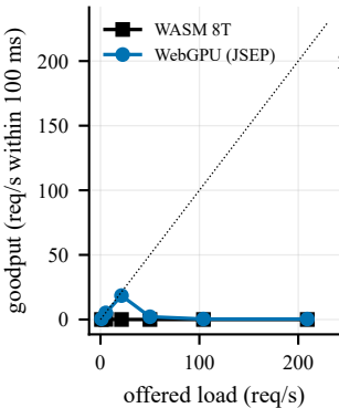
BERT-base
